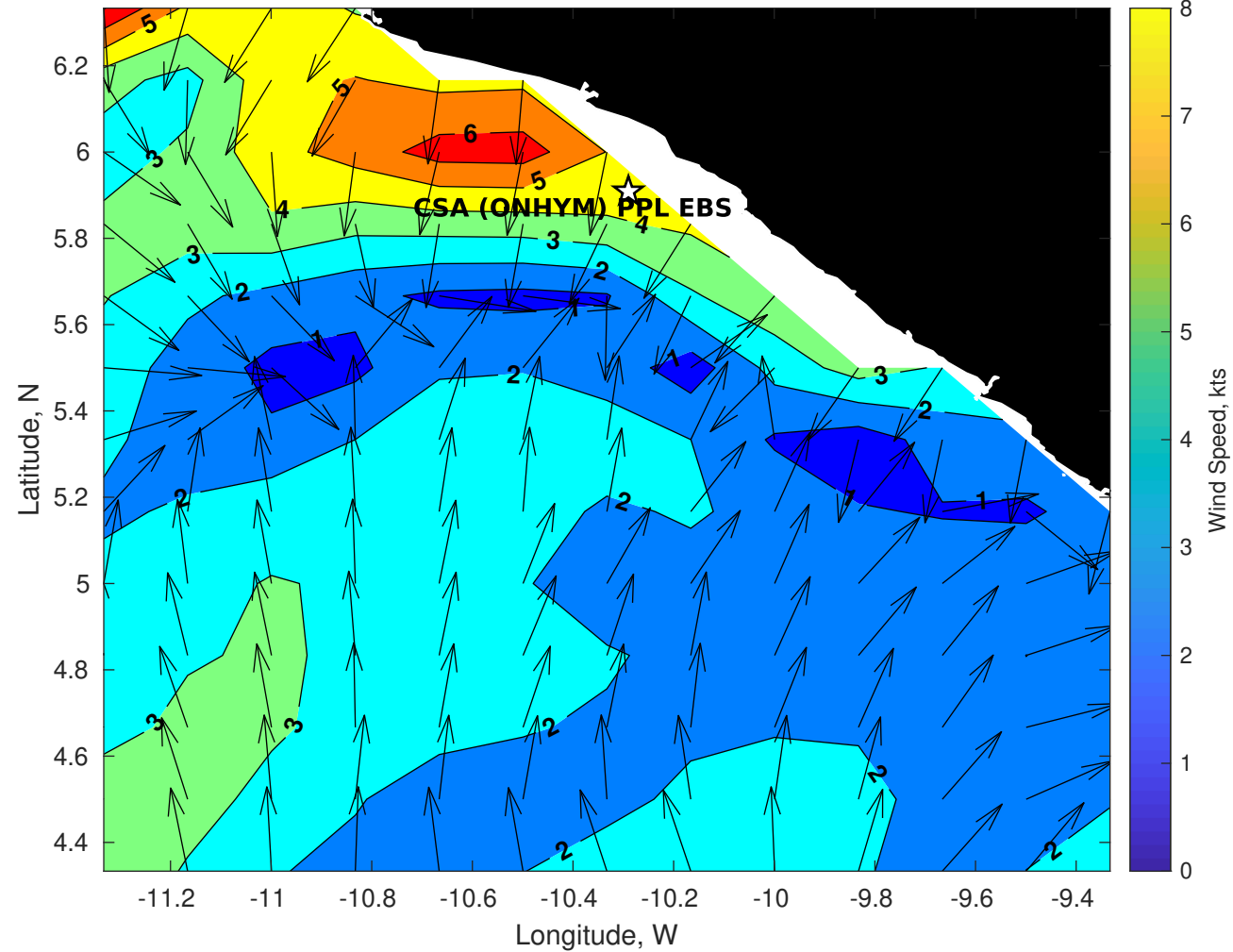
GFS Winds (kts) for CSA (ONHYM) PPL EBS - Liberia at 17-Dec-2025 09:00:00
