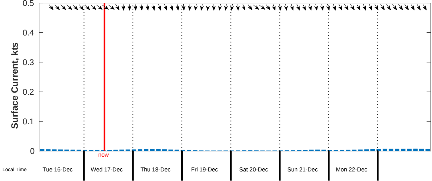
Surface Current Forecast for CSA (ONHYM) PPL EBS - Liberia from 16-Dec-2025 00:00:00 to 24-Dec-2025 00:00:00
