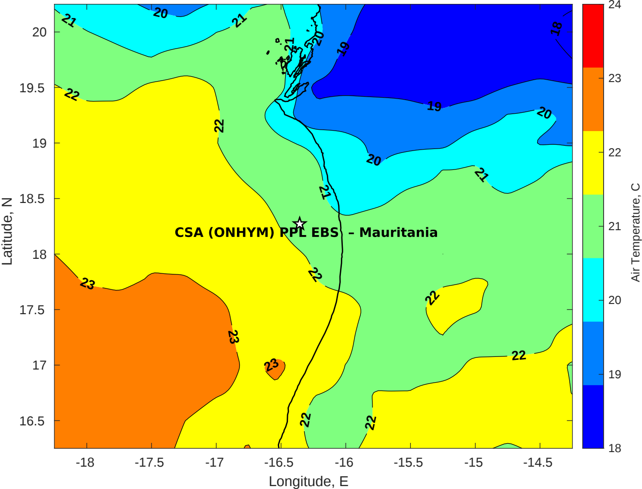
Air Temperature (C) for CSA (ONHYM) PPL EBS - Mauritania at 17-Dec-2025
