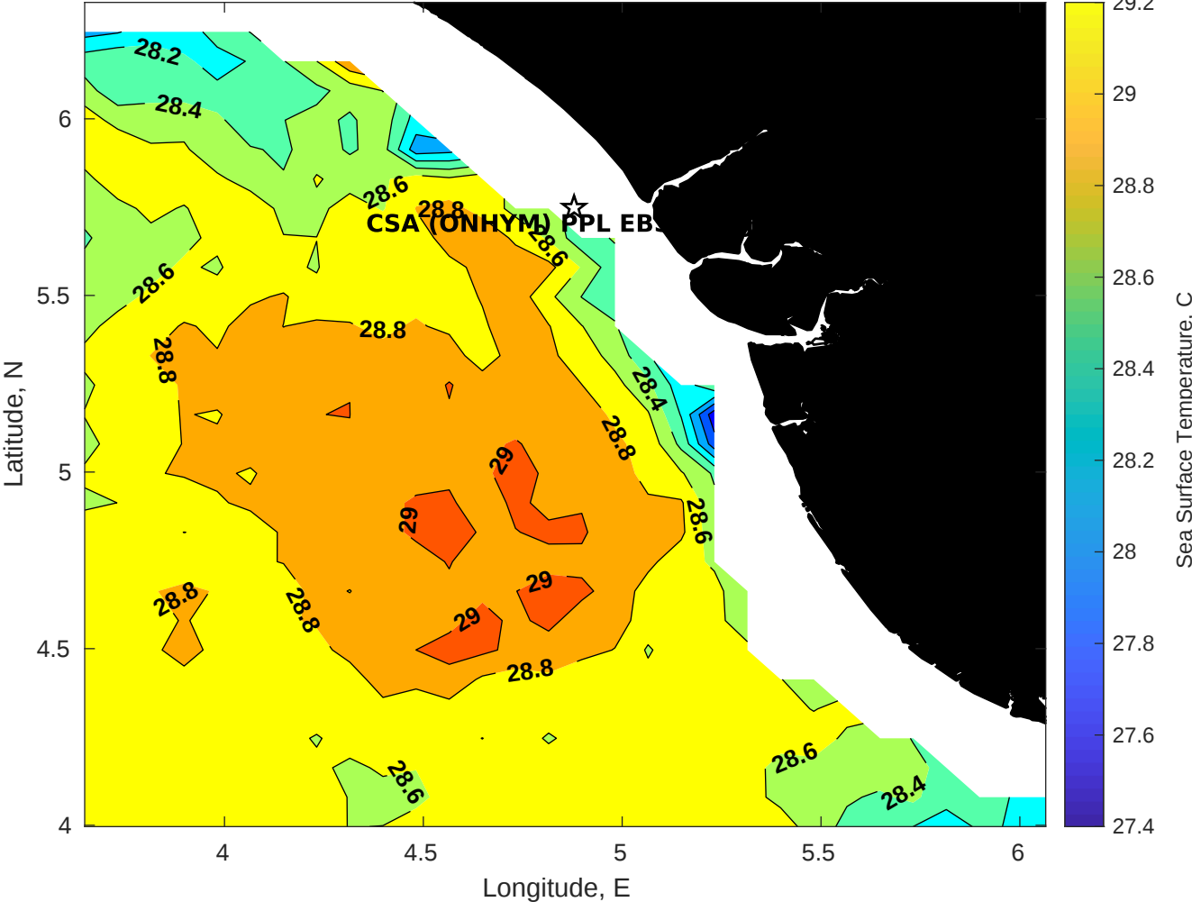
SST for CSA (ONHYM) PPL EBS - Nigeria at 16-Dec-2025 00:00:00
