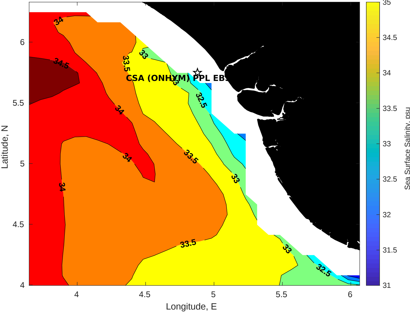
Surface Salinity for CSA (ONHYM) PPL EBS - Nigeria at 16-Dec-2025 00:00:00
