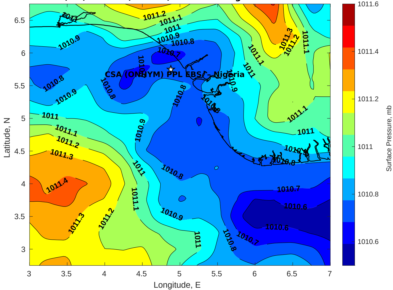
Surface Pressure (mb) for CSA (ONHYM) PPL EBS - Nigeria at 19-Dec-2025 00:00:00
