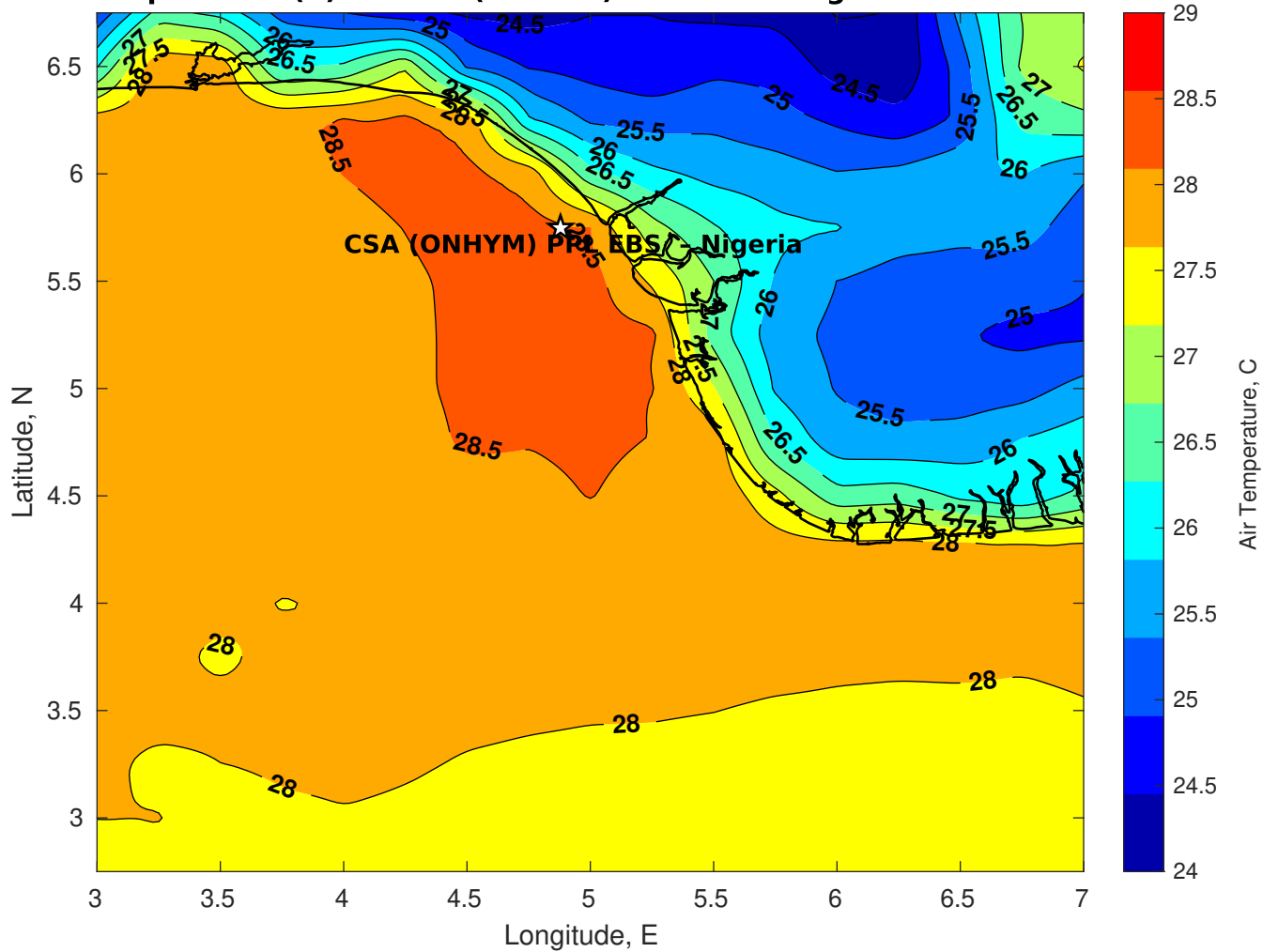
Air Temperature (C) for CSA (ONHYM) PPL EBS - Nigeria at 17-Dec-2025
