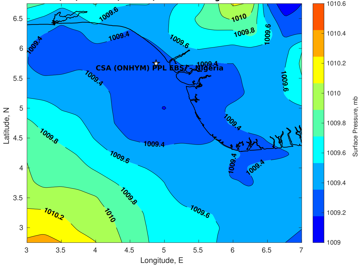
Surface Pressure (mb) for CSA (ONHYM) PPL EBS - Nigeria at 17-Dec-2025 00:00:00
