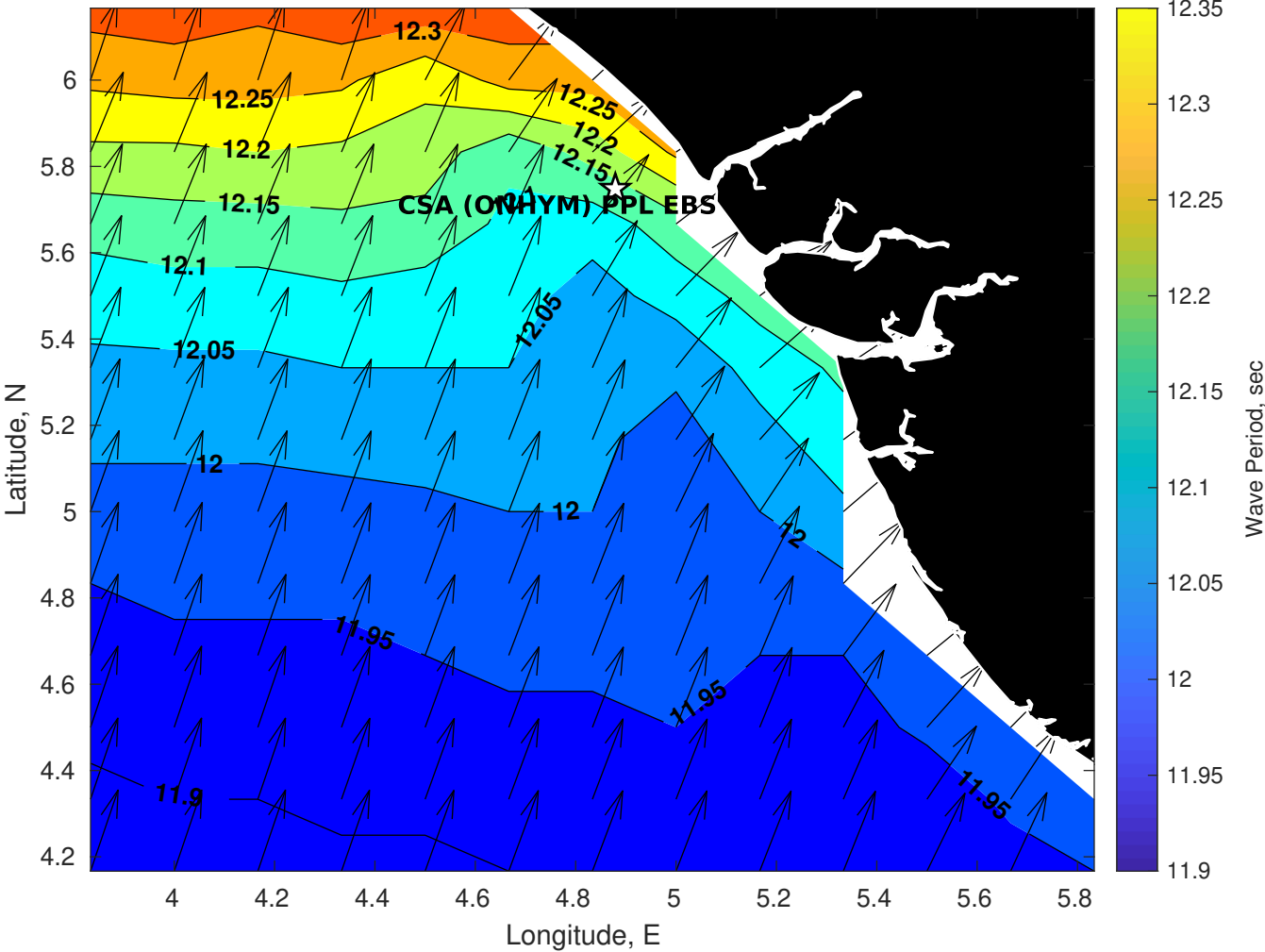
GFS Wave Period (sec) for CSA (ONHYM) PPL EBS - Nigeria at 17-Dec-2025 09:00:00
