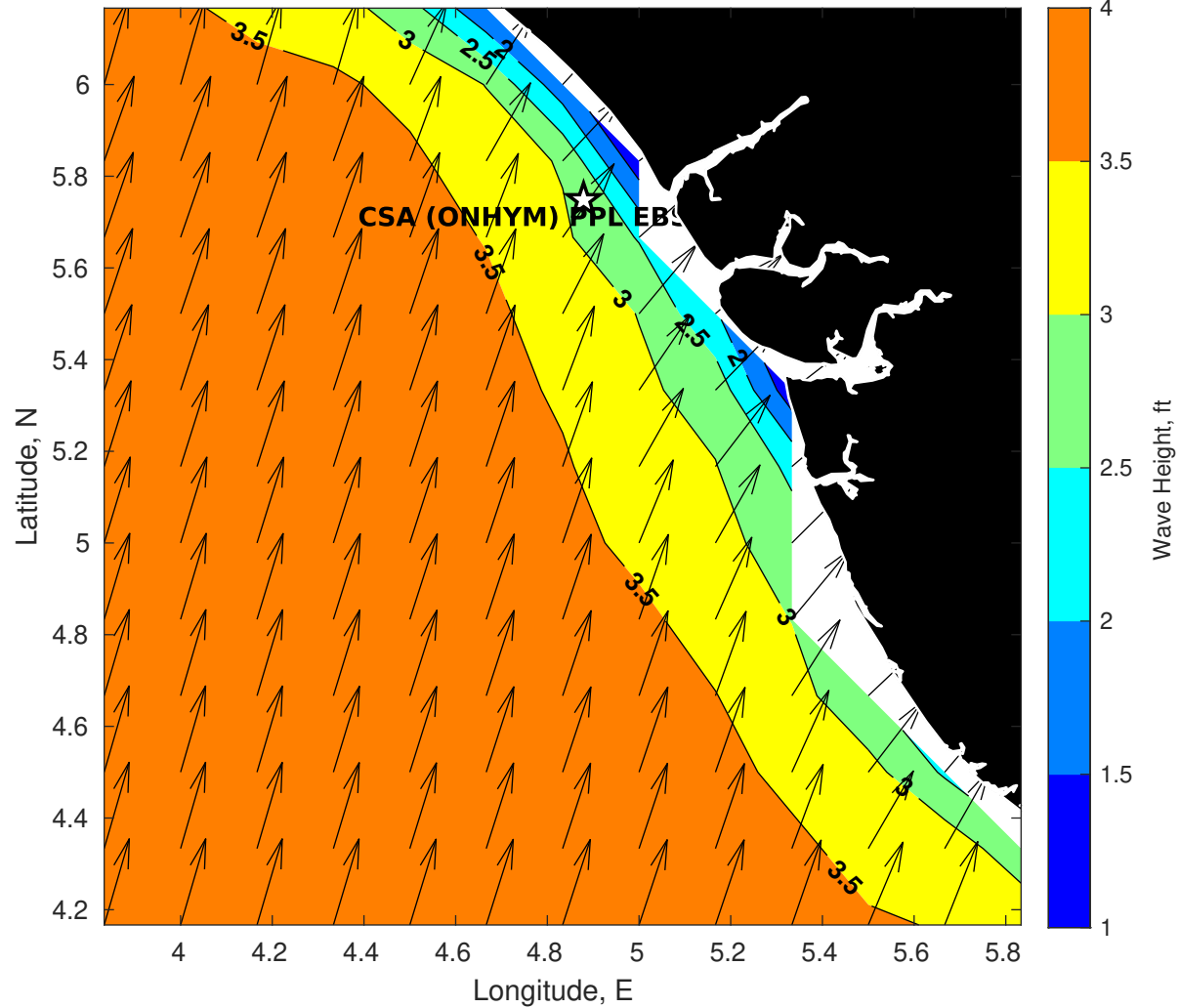
GFS Wave Height (ft) for CSA (ONHYM) PPL EBS - Nigeria at 17-Dec-2025 09:00:00
