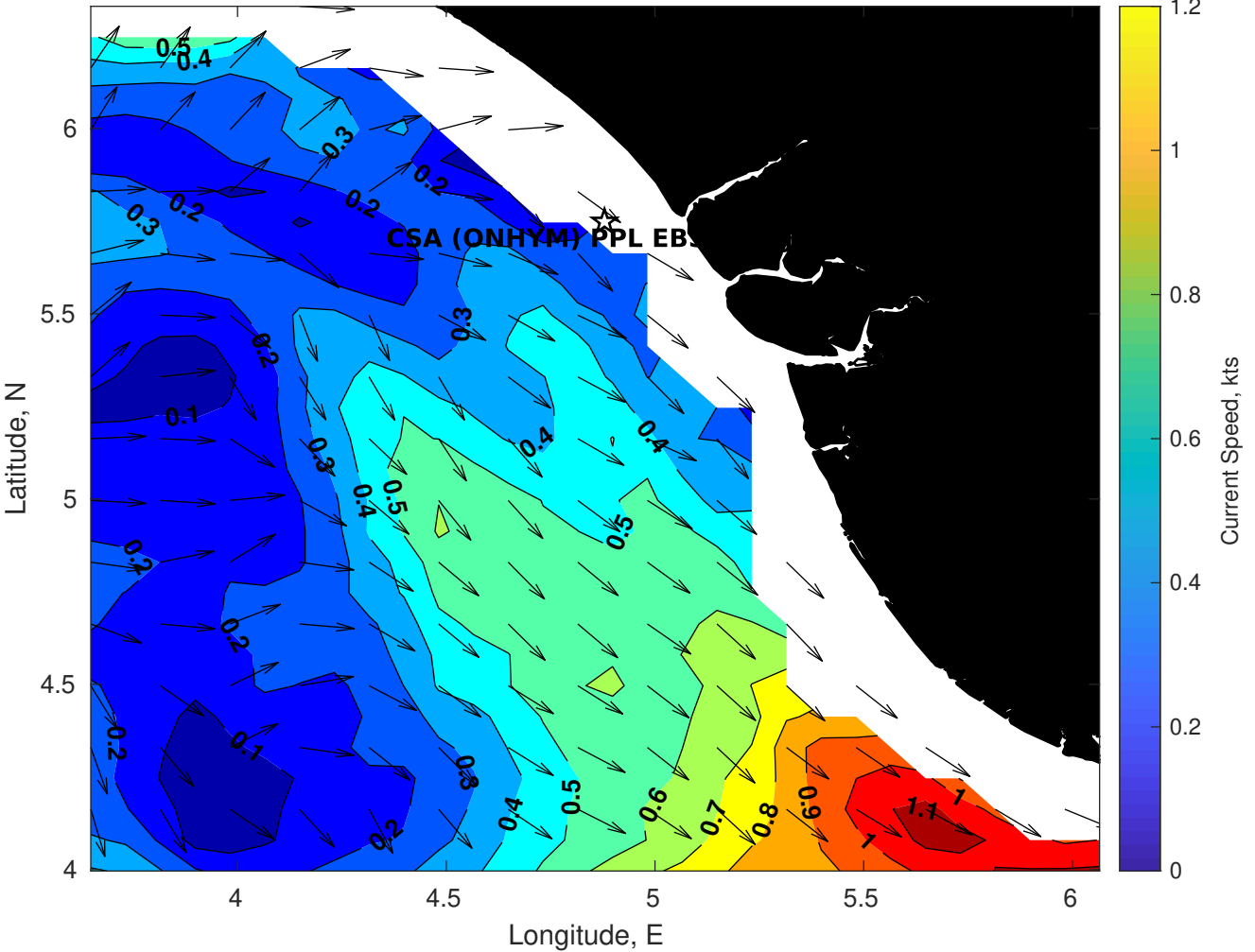
Surface Currents for CSA (ONHYM) PPL EBS - Nigeria at 16-Dec-2025 00:00:00
