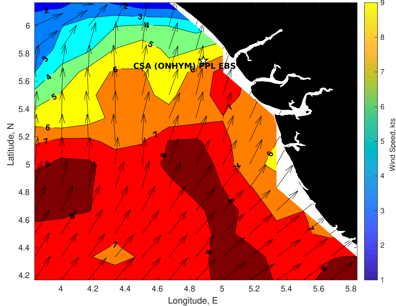
GFS Winds (kts) for CSA (ONHYM) PPL EBS - Nigeria at 17-Dec-2025 09:00:00
