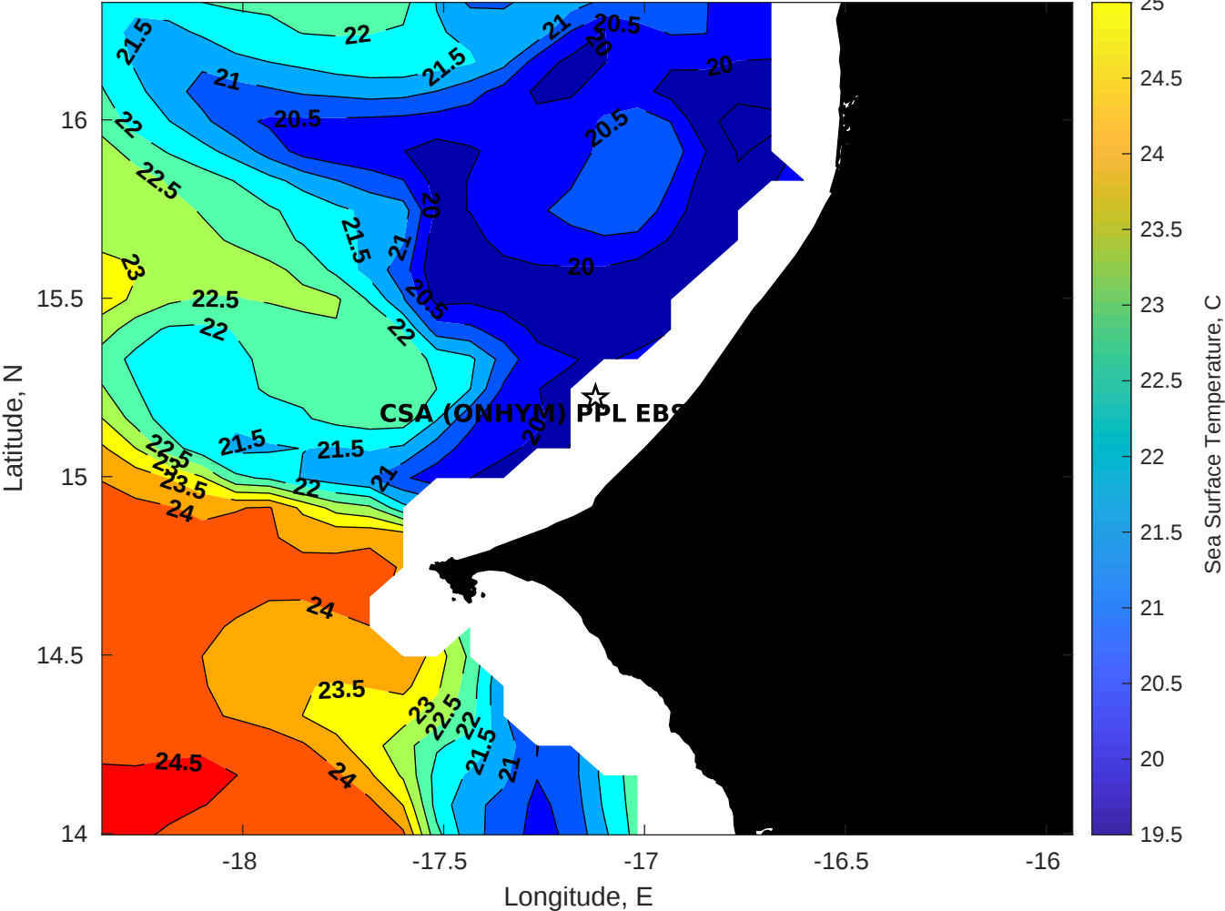
SST for CSA (ONHYM) PPL EBS - Senegal at 16-Dec-2025 00:00:00
