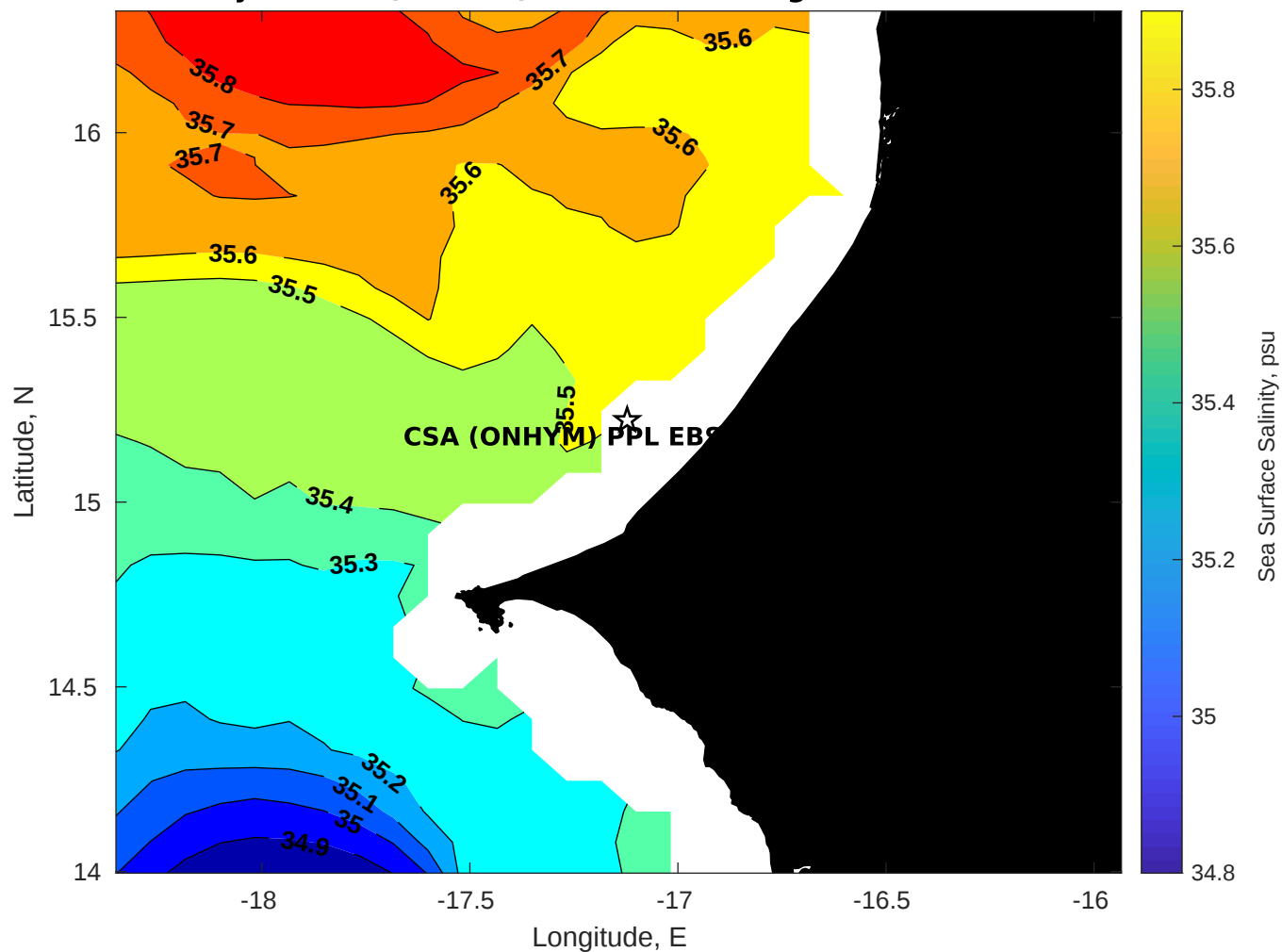
Surface Salinity for CSA (ONHYM) PPL EBS - Senegal at 16-Dec-2025 00:00:00
