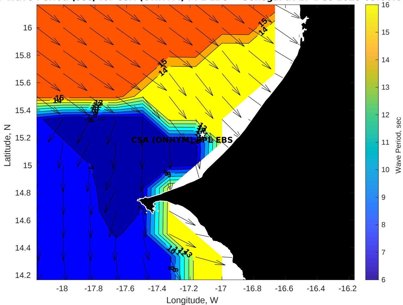
GFS Wave Period (sec) for CSA (ONHYM) PPL EBS - Senegal at 17-Dec-2025 09:00:00
