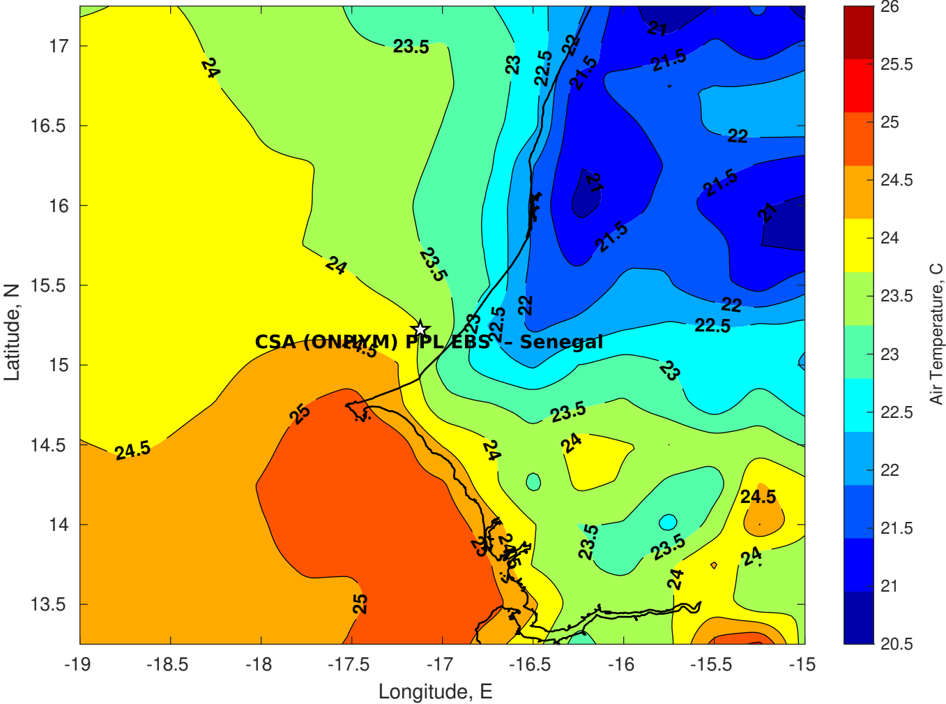
Air Temperature (C) for CSA (ONHYM) PPL EBS - Senegal at 17-Dec-2025
