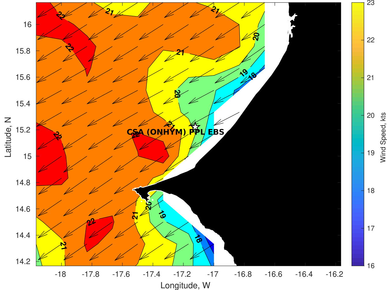
GFS Winds (kts) for CSA (ONHYM) PPL EBS - Senegal at 17-Dec-2025 09:00:00
