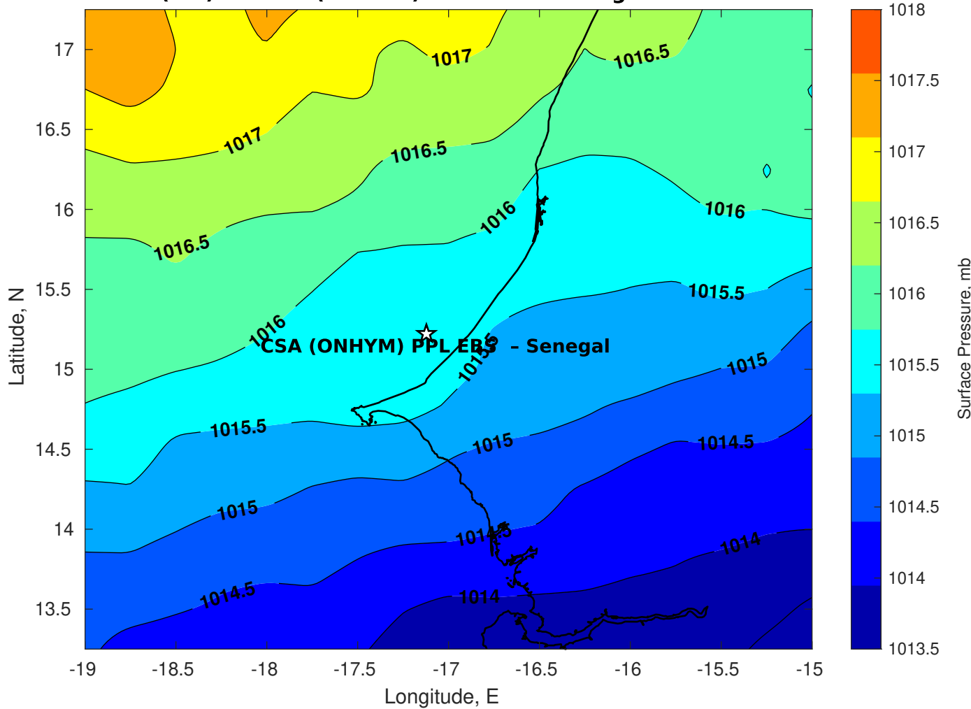
Surface Pressure (mb) for CSA (ONHYM) PPL EBS - Senegal at 19-Dec-2025 00:00:00
