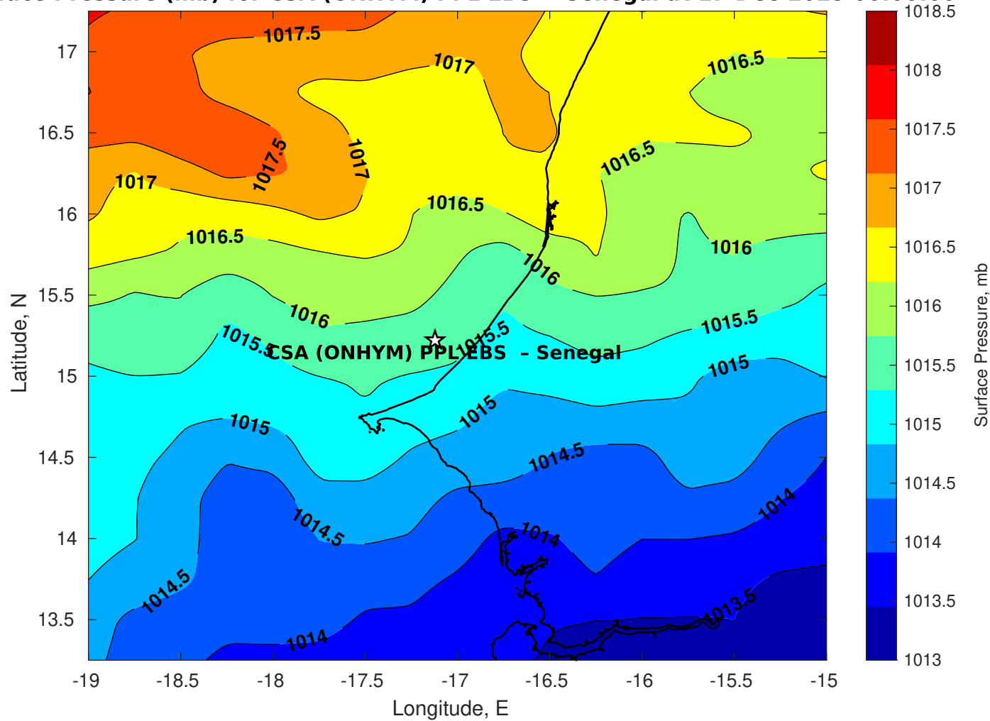
Surface Pressure (mb) for CSA (ONHYM) PPL EBS - Senegal at 17-Dec-2025 00:00:00
