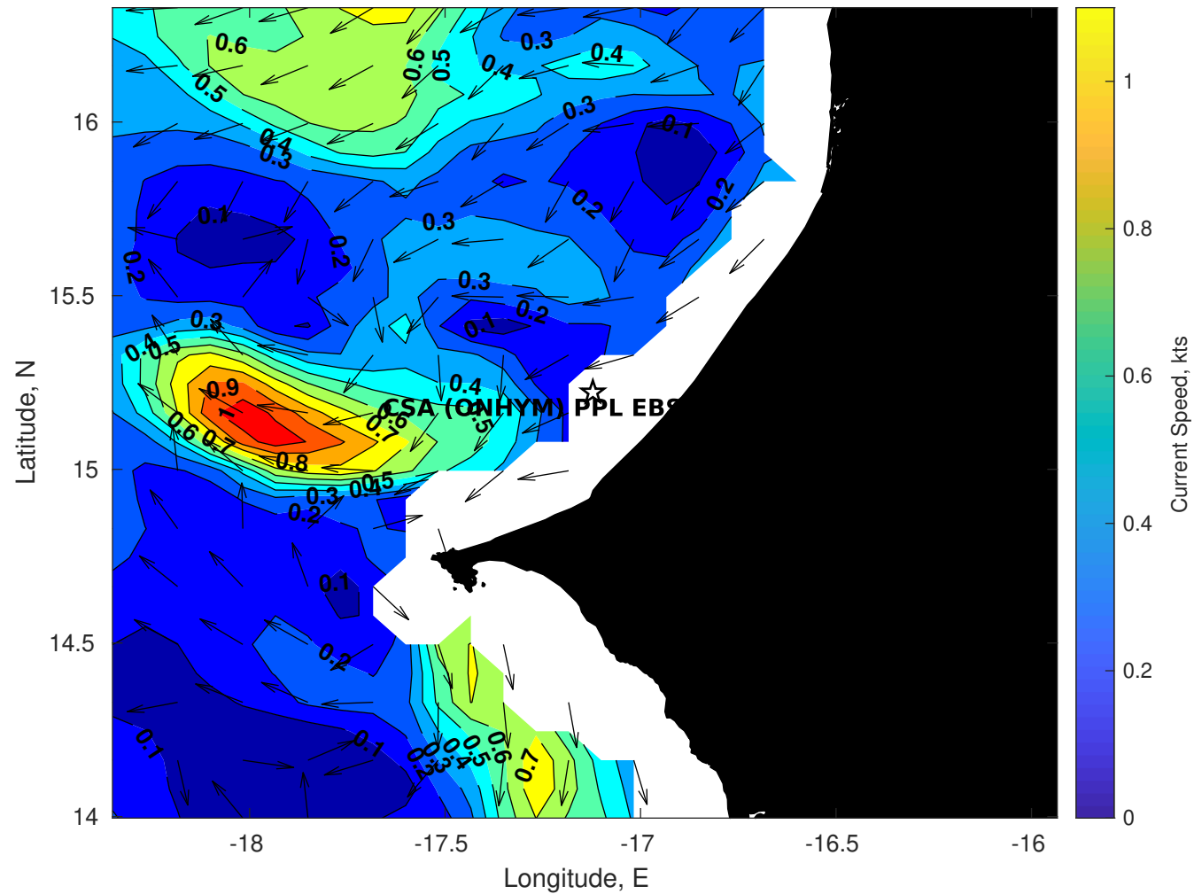
Surface Currents for CSA (ONHYM) PPL EBS - Senegal at 16-Dec-2025 00:00:00
