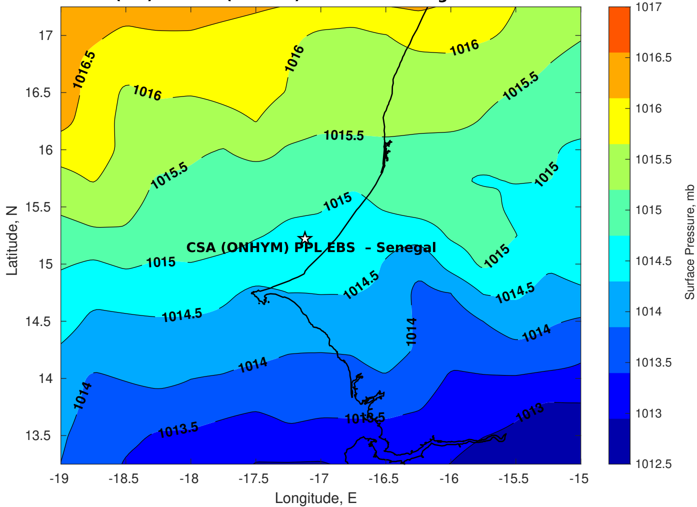
Surface Pressure (mb) for CSA (ONHYM) PPL EBS - Senegal at 18-Dec-2025 00:00:00
