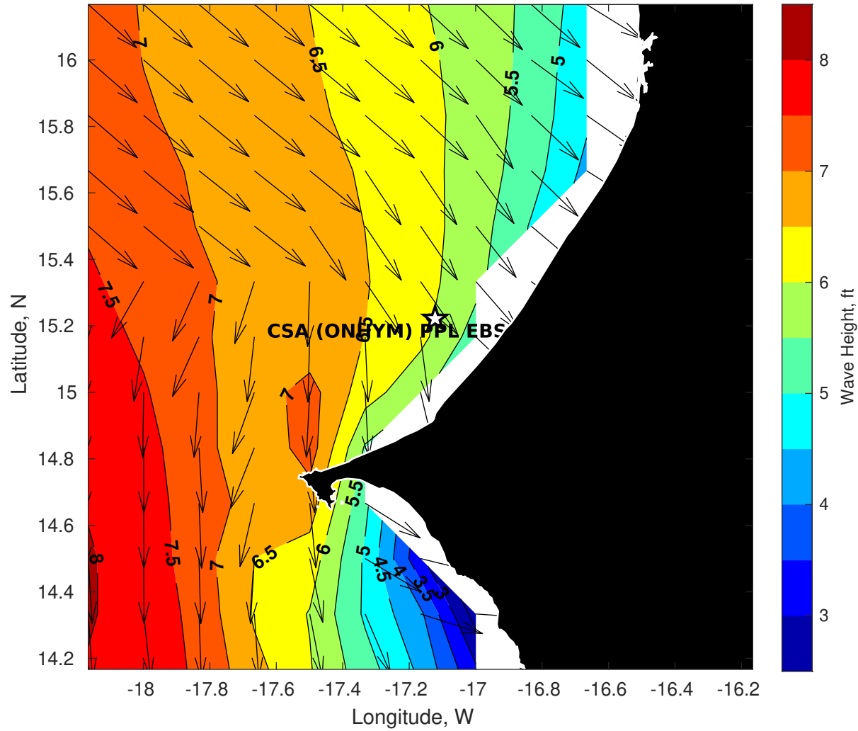
GFS Wave Height (ft) for CSA (ONHYM) PPL EBS - Senegal at 17-Dec-2025 09:00:00
