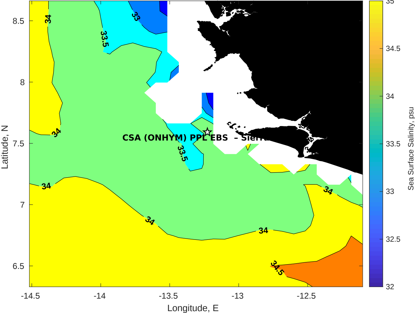
Surface Salinity for CSA (ONHYM) PPL EBS - Sierra Leone at 16-Dec-2025 00:00:00
