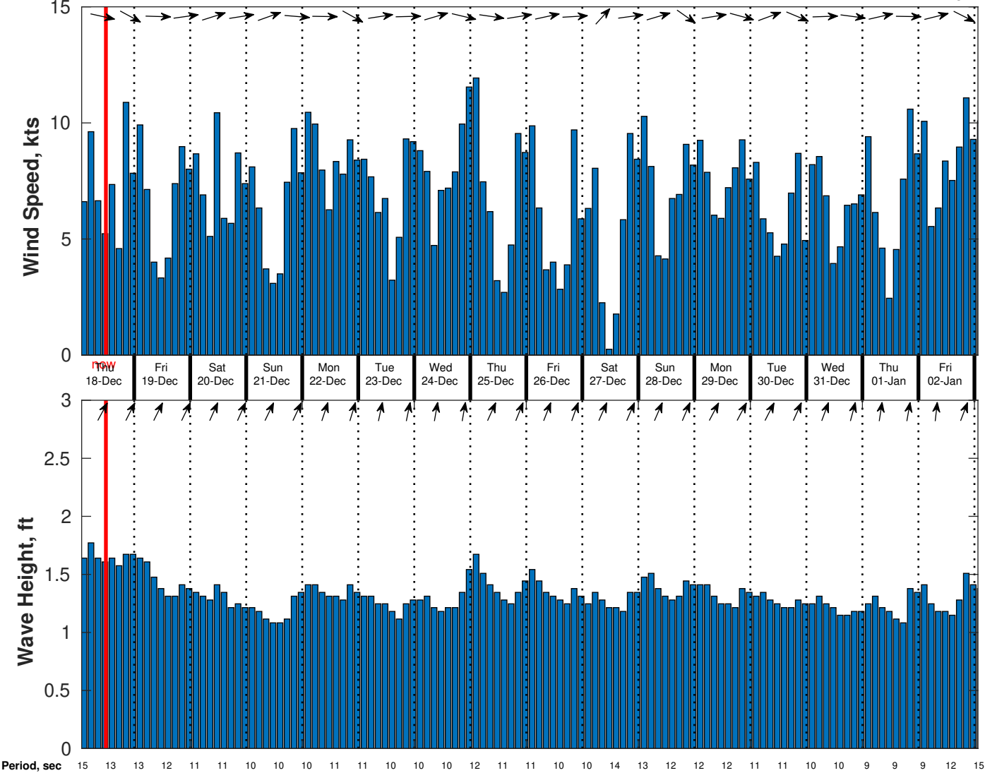
Wind & Wave Forecast for CSA (ONHYM) PPL EBS - Sierra Leone from 17-Dec-2025 01:00:00 to 02-Jan-2026 01:00:00
