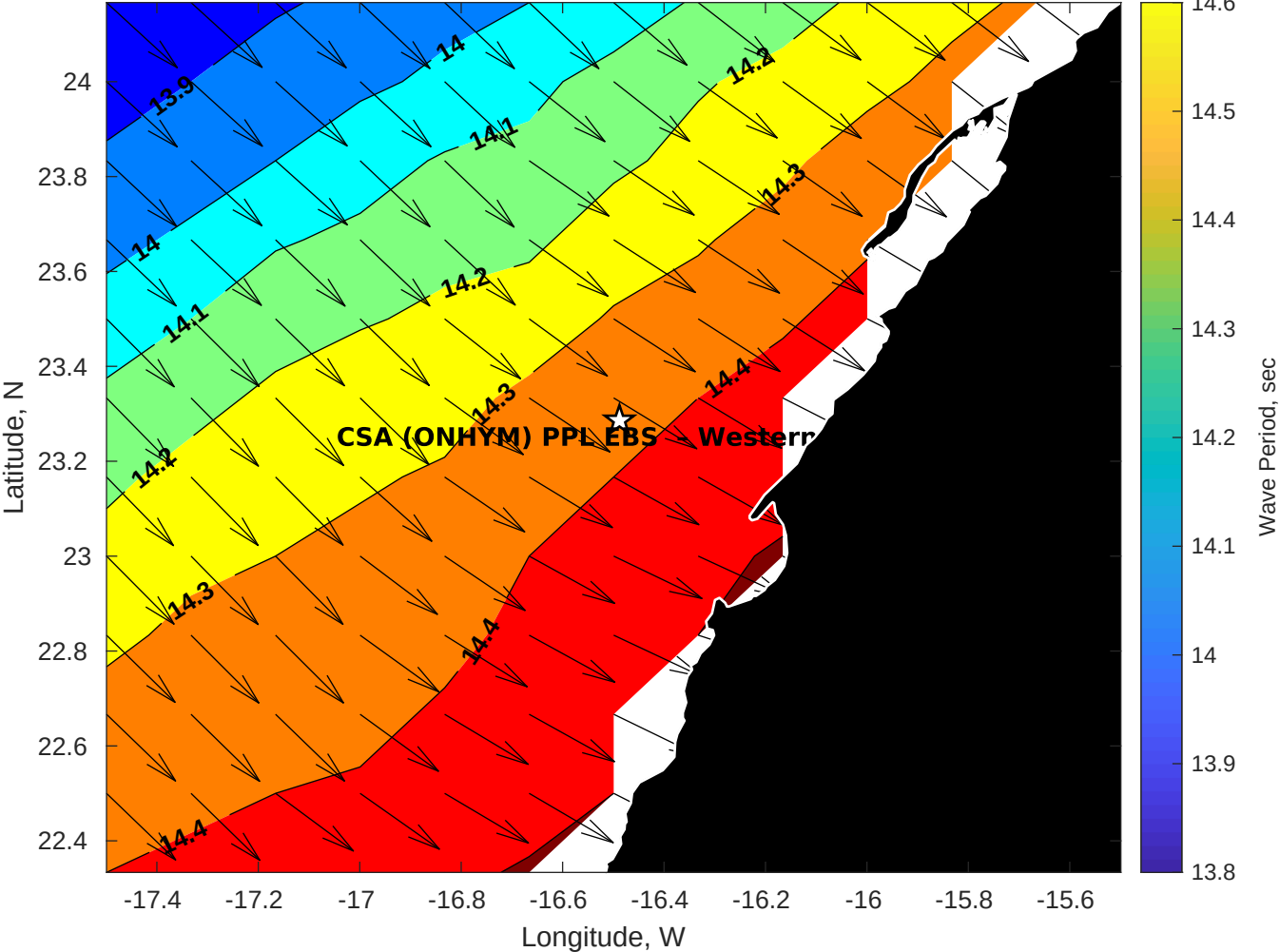
GFS Wave Period (sec) for CSA (ONHYM) PPL EBS - Western Sahara at 17-Dec-2025 09:00:00
