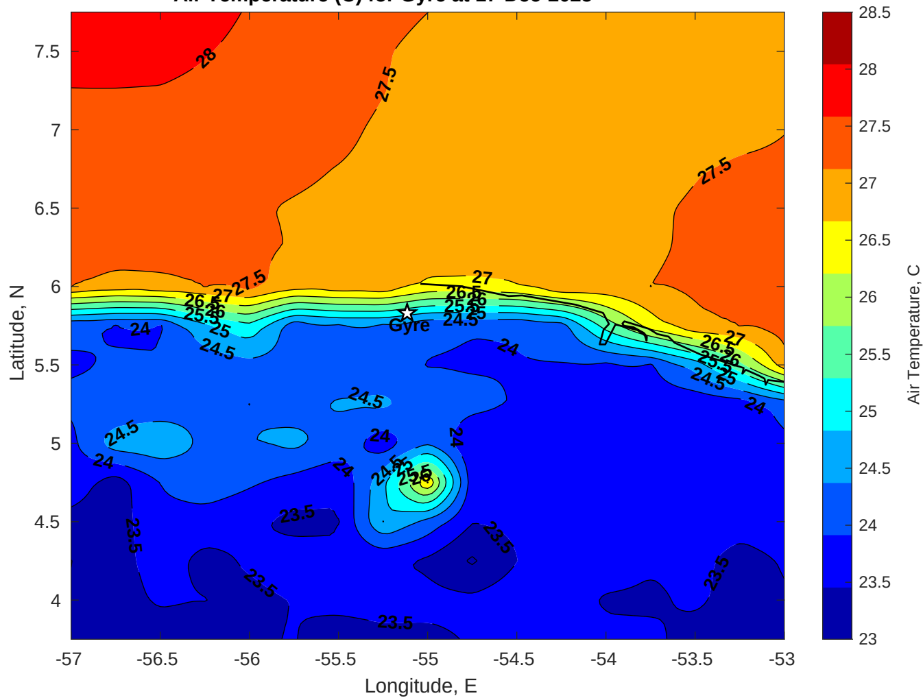
Air Temperature (C) for Gyre at 17-Dec-2025
