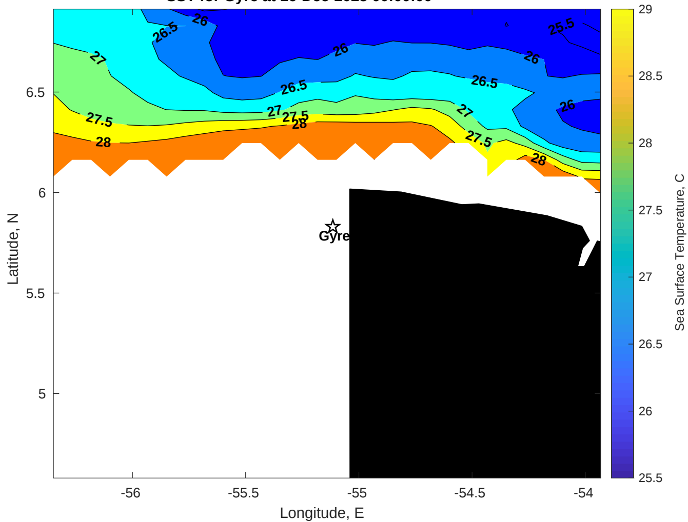
SST for Gyre at 16-Dec-2025 00:00:00
