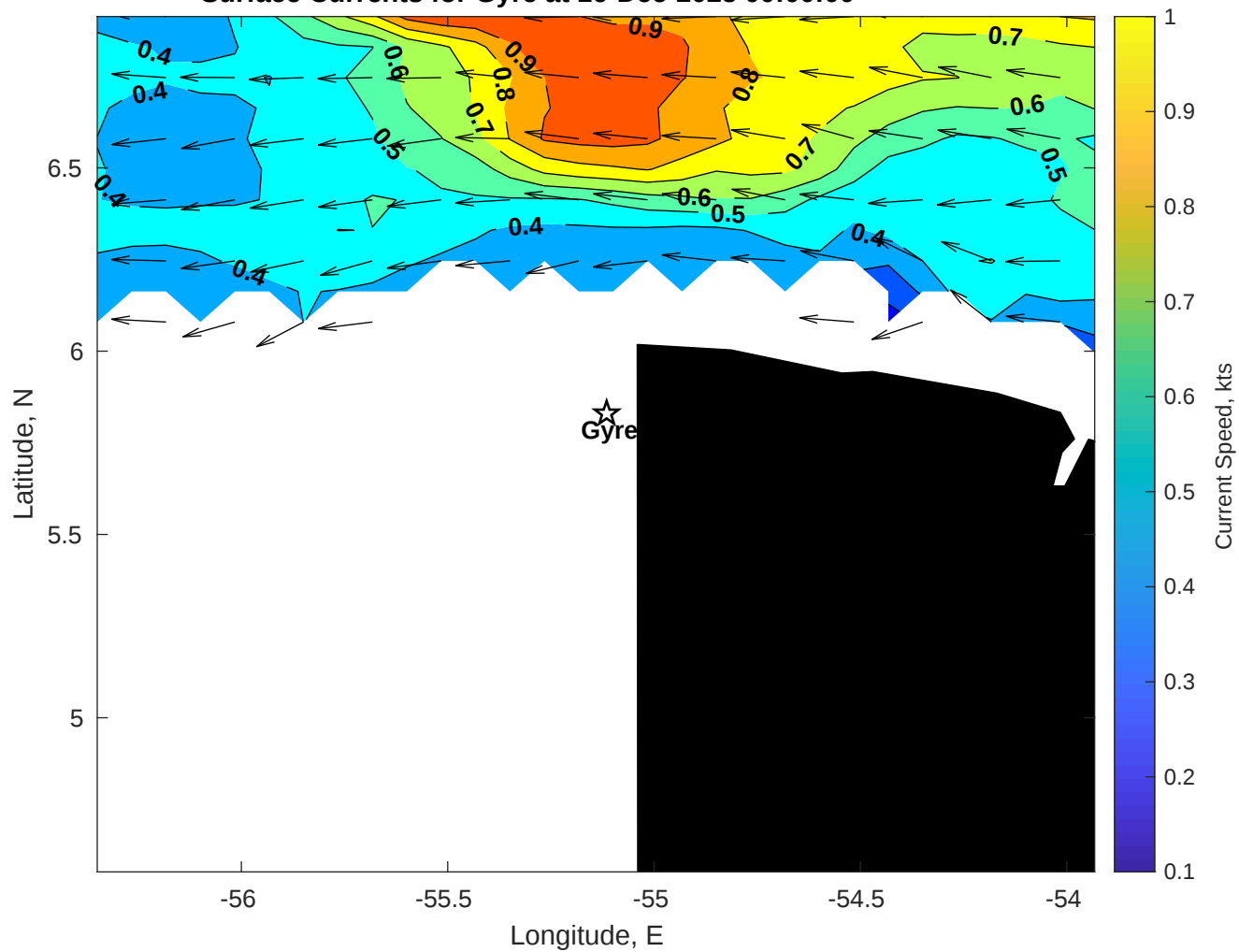
Surface Currents for Gyre at 16-Dec-2025 00:00:00
