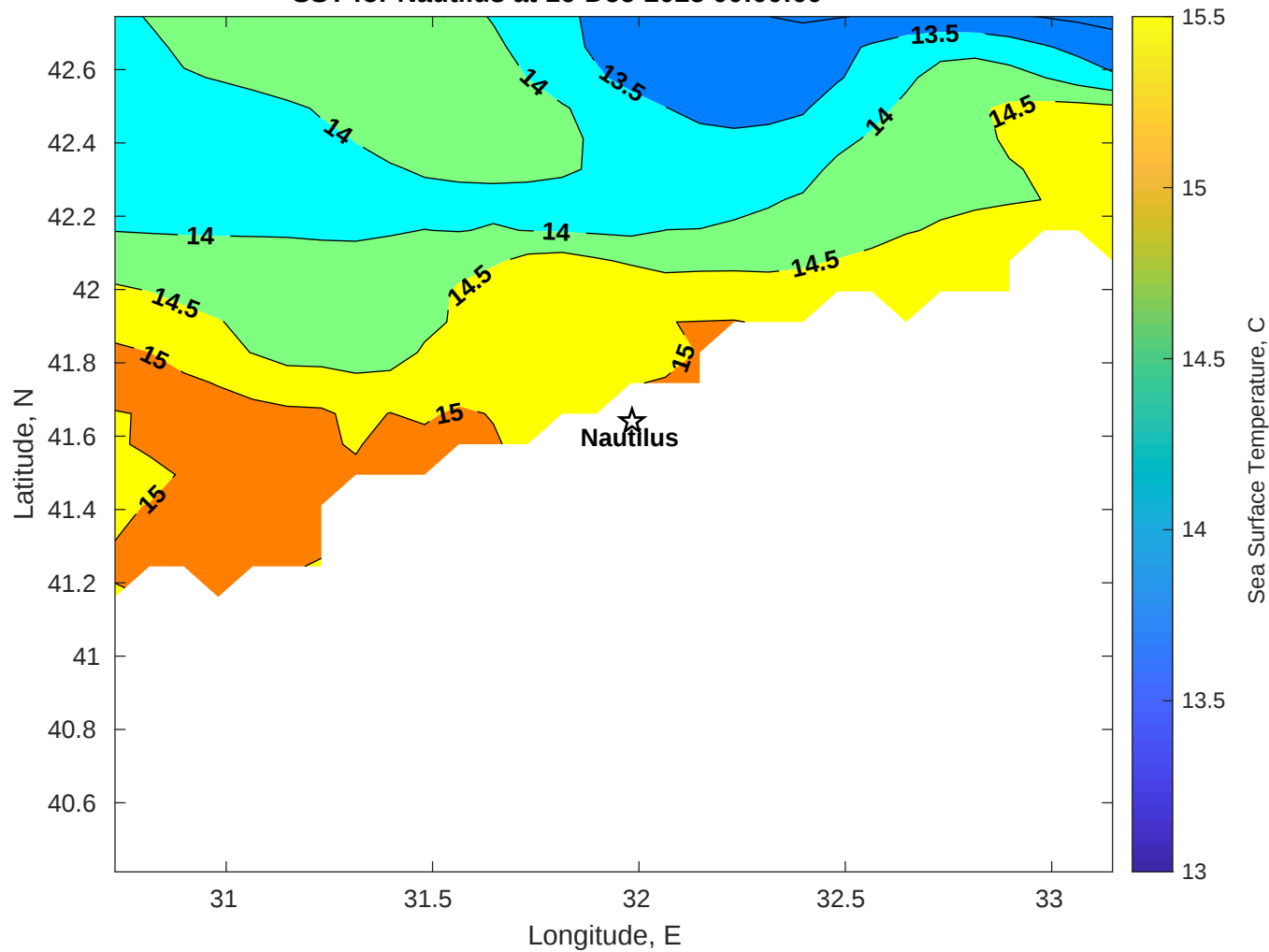
SST for Nautilus at 16-Dec-2025 00:00:00
