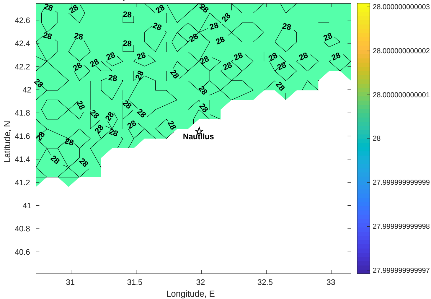
Surface Salinity for Nautilus at 16-Dec-2025 00:00:00
