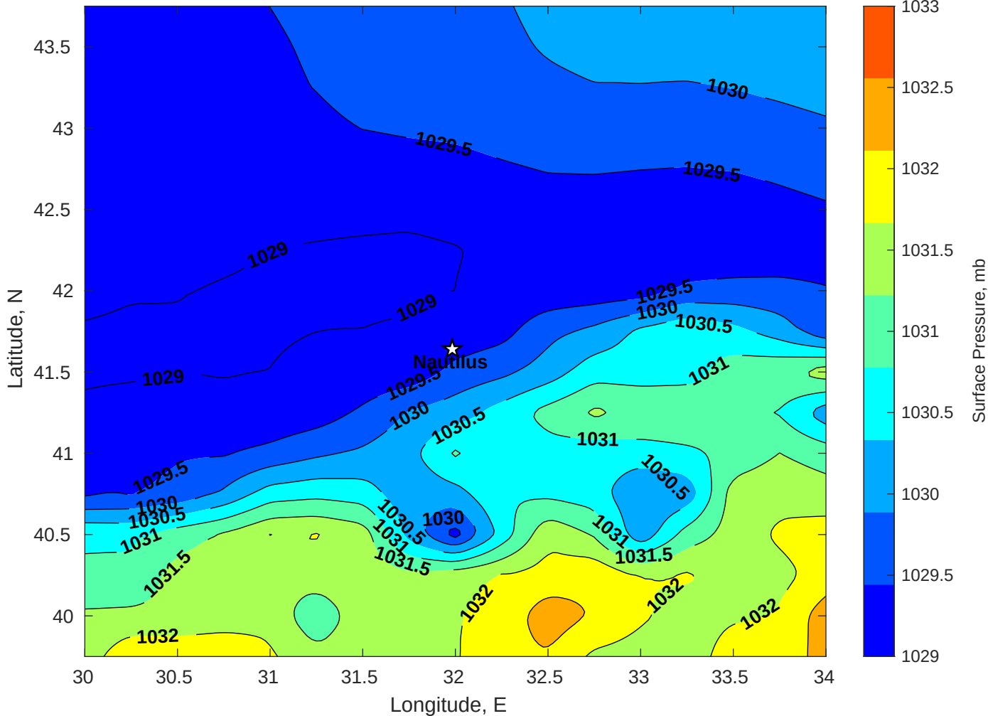
Surface Pressure (mb) for Nautilus at 18-Dec-2025 00:00:00
