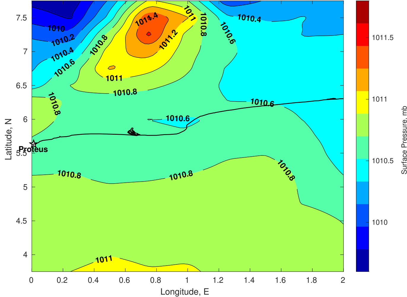
Surface Pressure (mb) for Proteus at 18-Dec-2025 00:00:00
