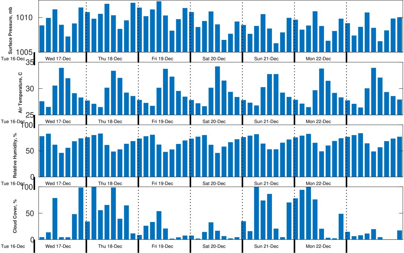
Met Forecast for Proteus from 17-Dec-2025 00:00:00 to 24-Dec-2025 00:00:00
