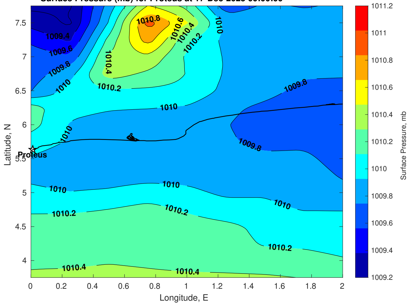
Surface Pressure (mb) for Proteus at 17-Dec-2025 00:00:00
