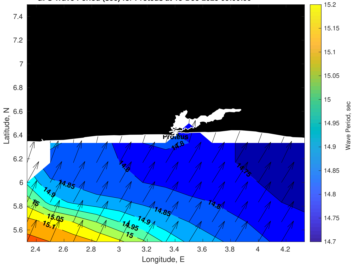
GFS Wave Period (sec) for Proteus at 15-Dec-2025 09:00:00
