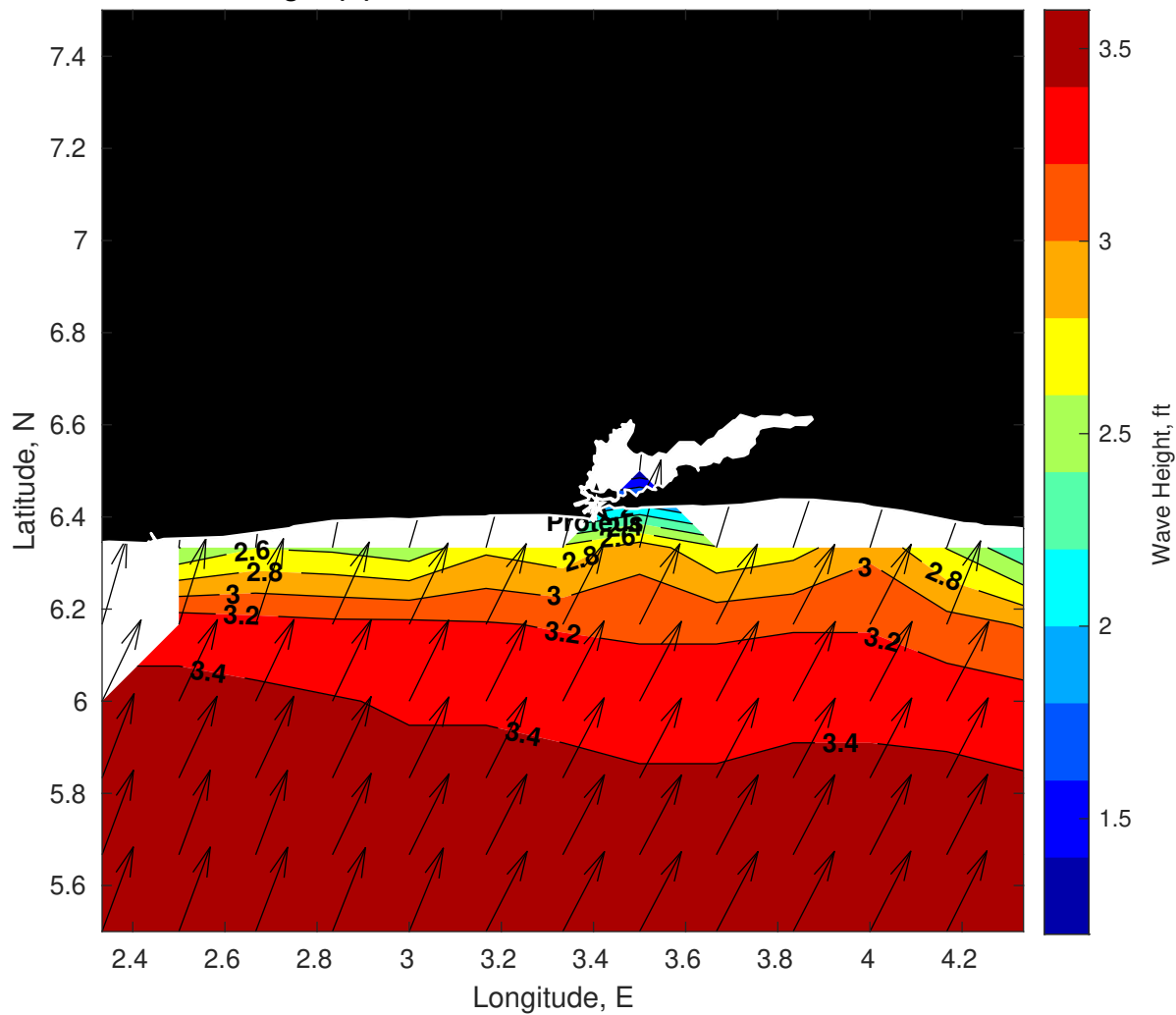
GFS Wave Height (ft) for Proteus at 15-Dec-2025 09:00:00
