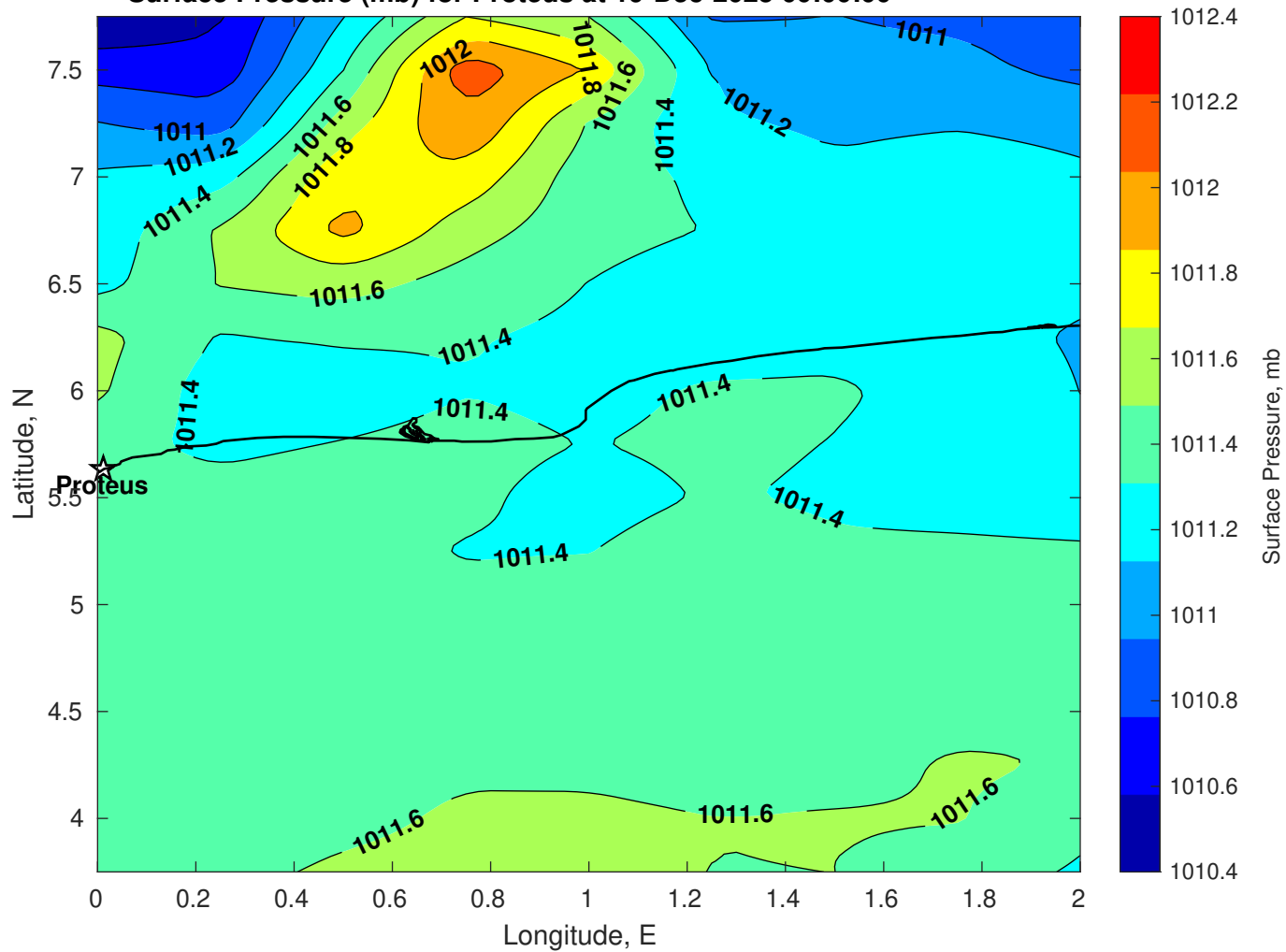
Surface Pressure (mb) for Proteus at 19-Dec-2025 00:00:00
