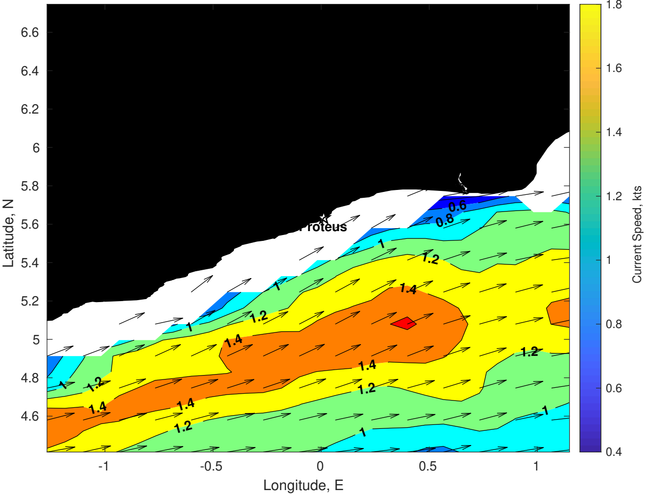
Surface Currents for Proteus at 16-Dec-2025 00:00:00
