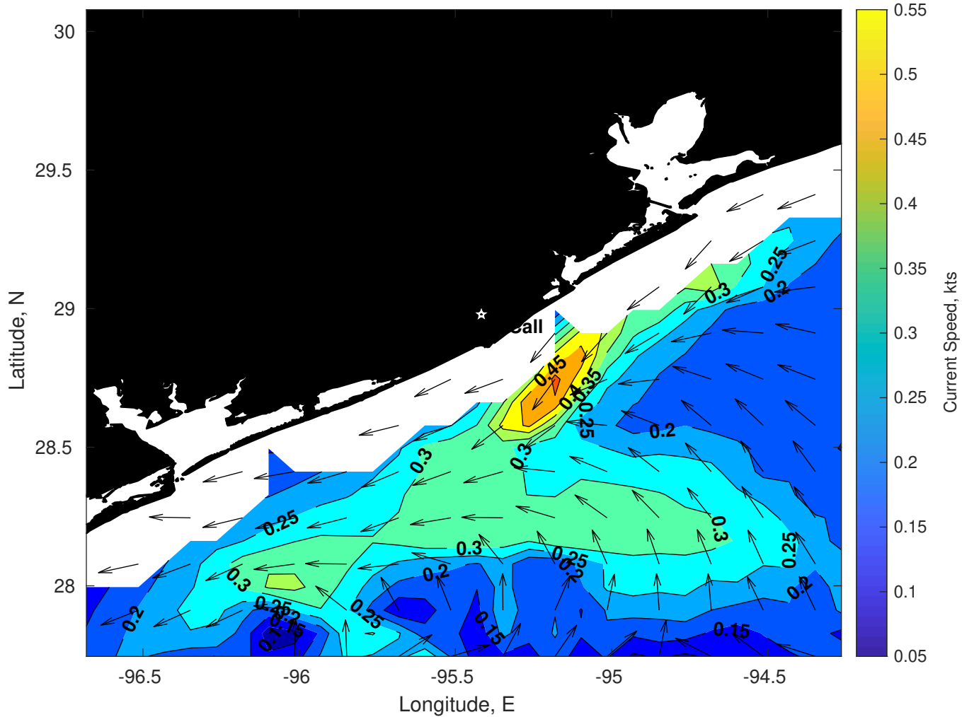
Surface Currents for Brooks McCall at 17-Dec-2025 00:00:00
