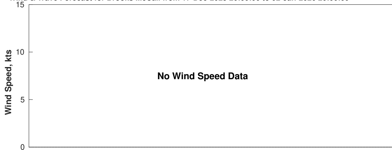
Wind & Wave Forecast for Brooks McCall from 17-Dec-2025 20:00:00 to 02-Jan-2026 20:00:00
