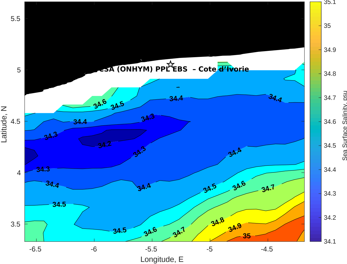
Surface Salinity for CSA (ONHYM) PPL EBS - Cote d'Ivoire at 17-Dec-2025 00:00:00
