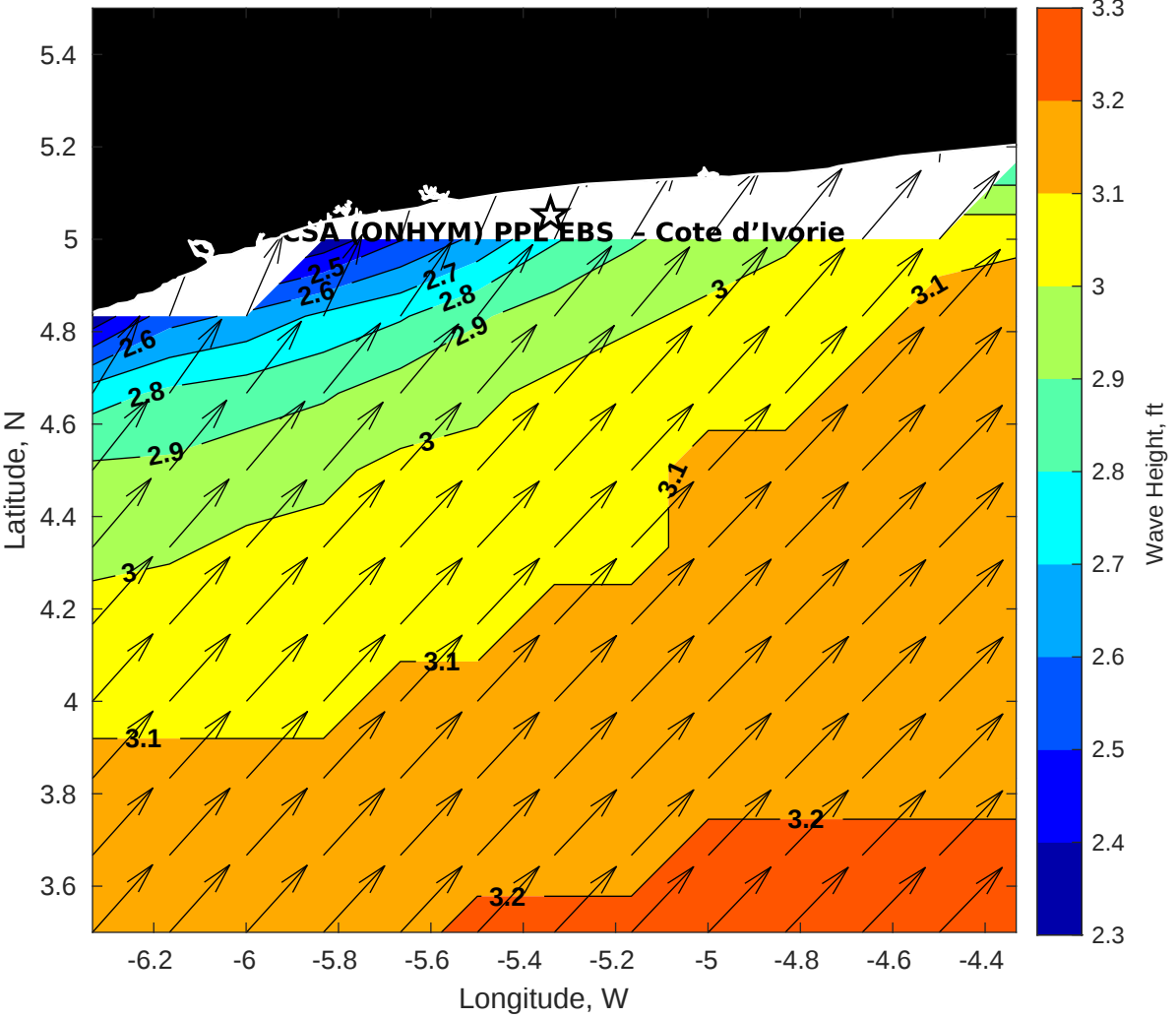
GFS Wave Height (ft) for CSA (ONHYM) PPL EBS - Cote d'Ivoire at 18-Dec-2025 09:00:00
