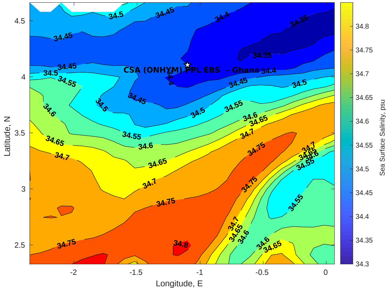
Surface Salinity for CSA (ONHYM) PPL EBS - Ghana at 17-Dec-2025 00:00:00
