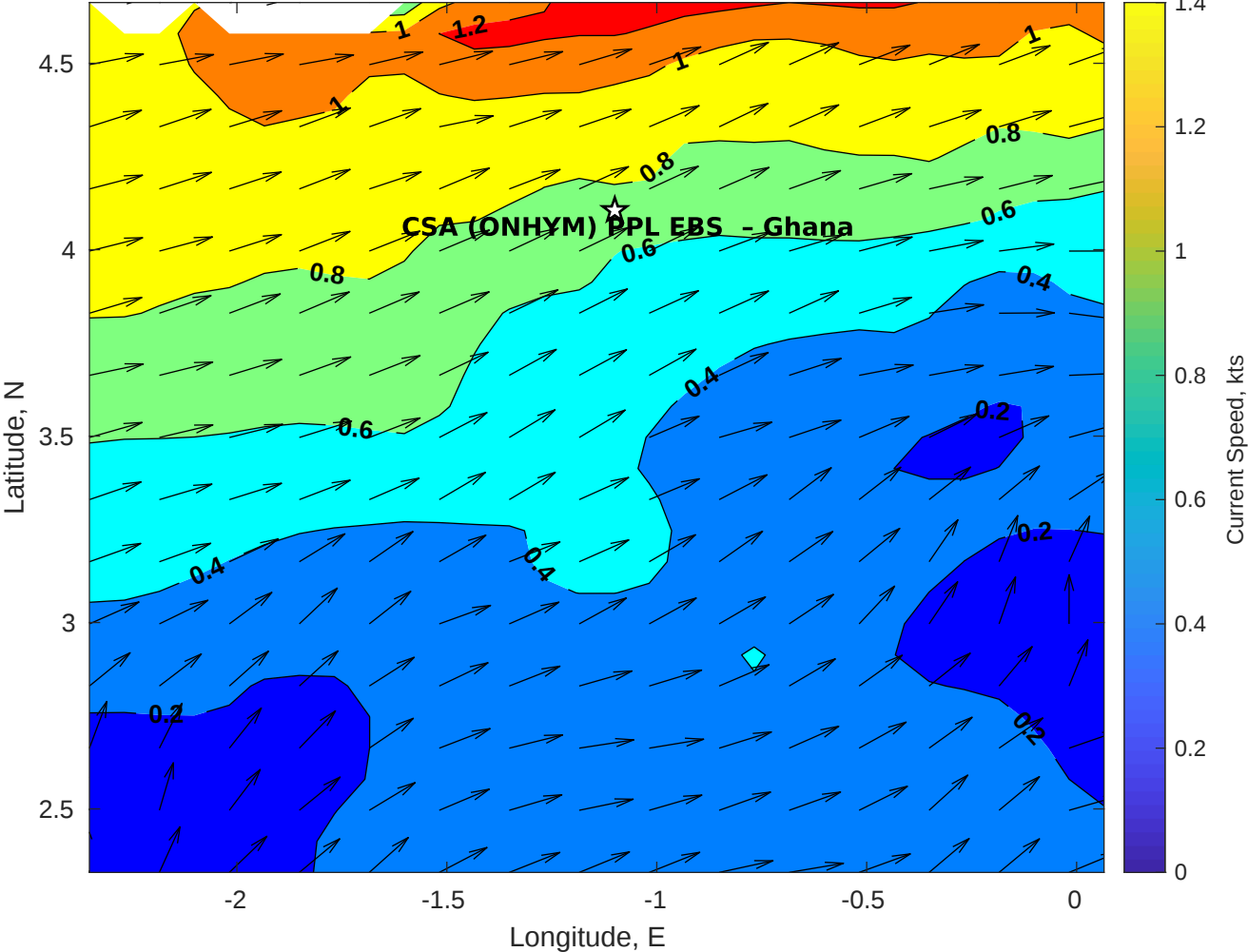
Surface Currents for CSA (ONHYM) PPL EBS - Ghana at 17-Dec-2025 00:00:00
