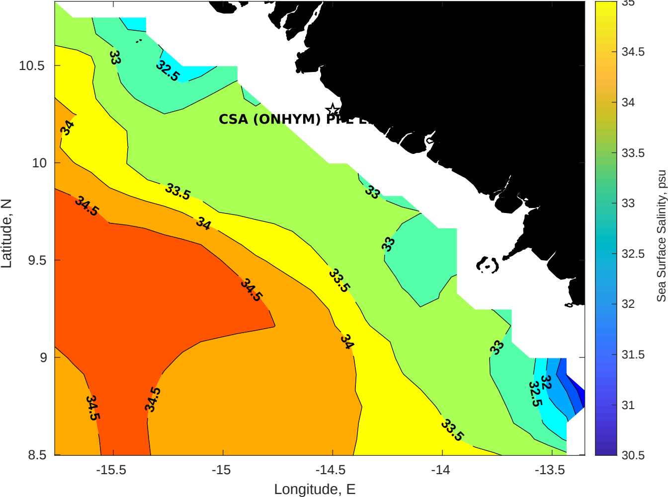
Surface Salinity for CSA (ONHYM) PPL EBS - Guinea at 17-Dec-2025 00:00:00
