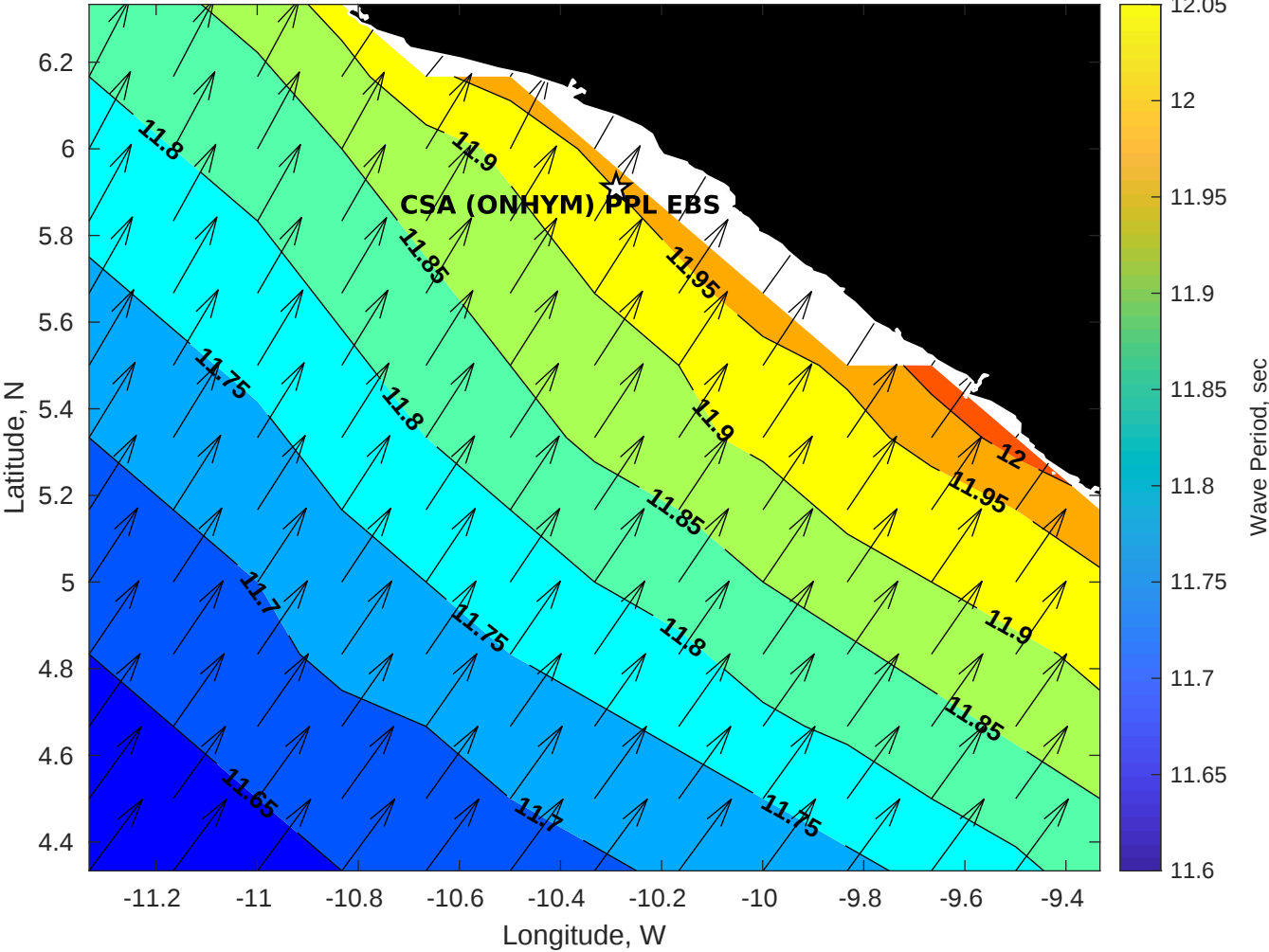
GFS Wave Period (sec) for CSA (ONHYM) PPL EBS - Liberia at 18-Dec-2025 09:00:00
