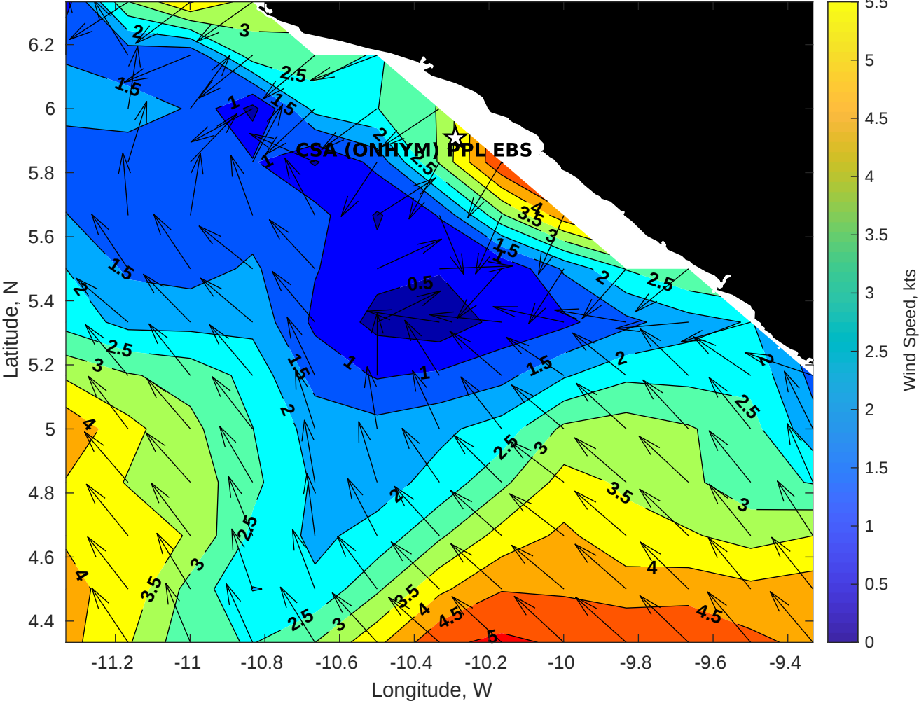
GFS Winds (kts) for CSA (ONHYM) PPL EBS - Liberia at 18-Dec-2025 09:00:00
