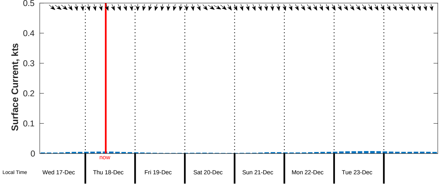
Surface Current Forecast for CSA (ONHYM) PPL EBS - Liberia from 17-Dec-2025 00:00:00 to 25-Dec-2025 00:00:00
