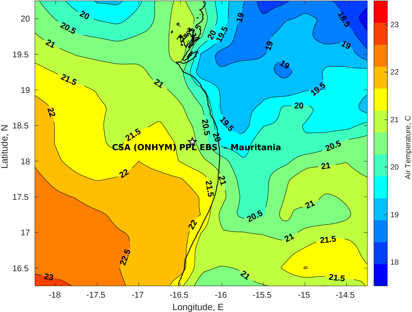
Air Temperature (C) for CSA (ONHYM) PPL EBS - Mauritania at 18-Dec-2025
