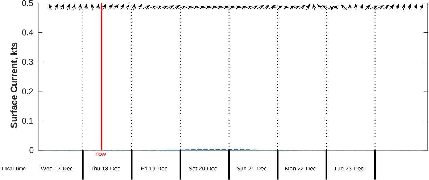
Surface Current Forecast for CSA (ONHYM) PPL EBS - Mauritania from 17-Dec-2025 00:00:00 to 25-Dec-2025 00:00:00
