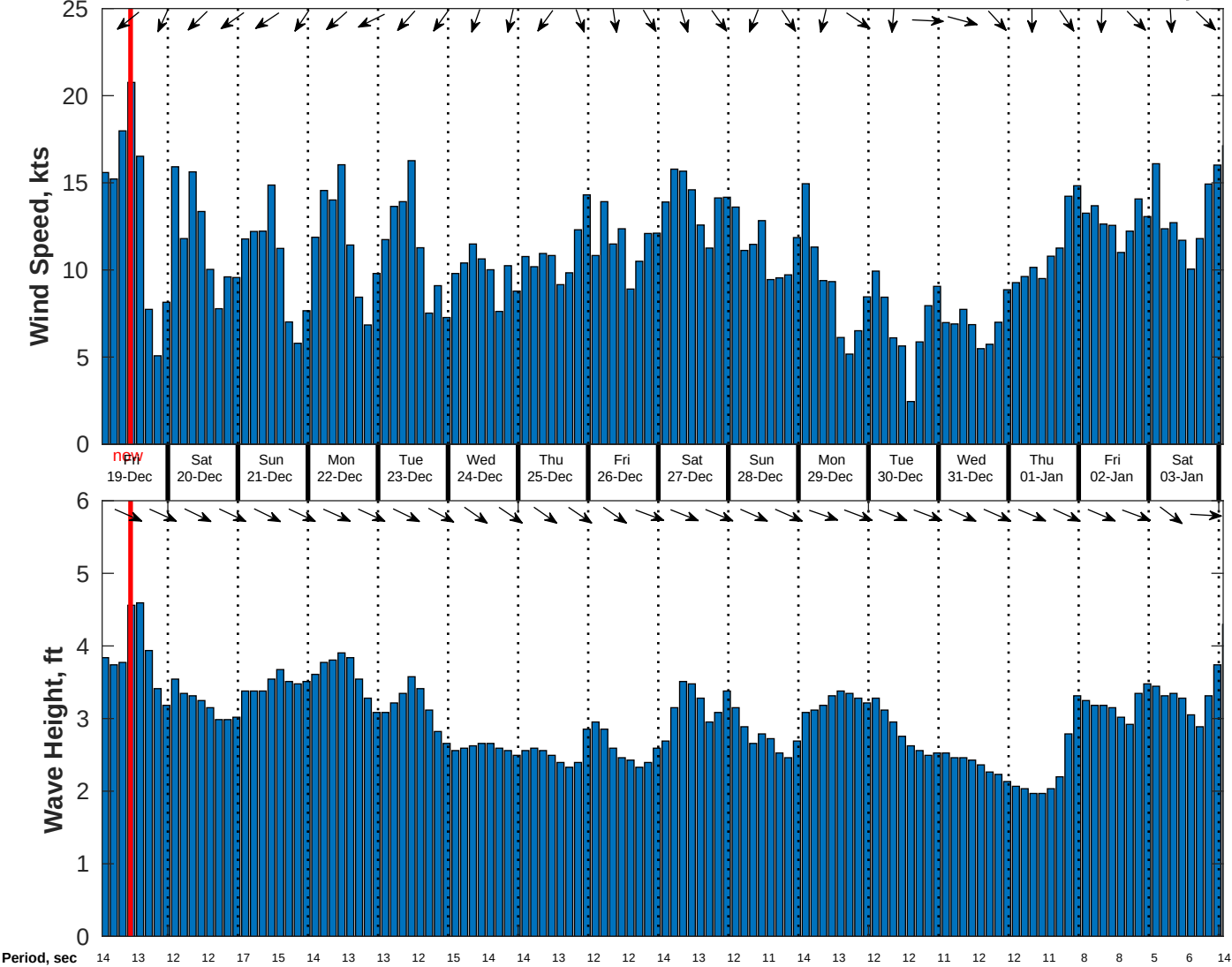
Wind & Wave Forecast for CSA (ONHYM) PPL EBS - Mauritania from 18-Dec-2025 01:00:00 to 03-Jan-2026 01:00:00
