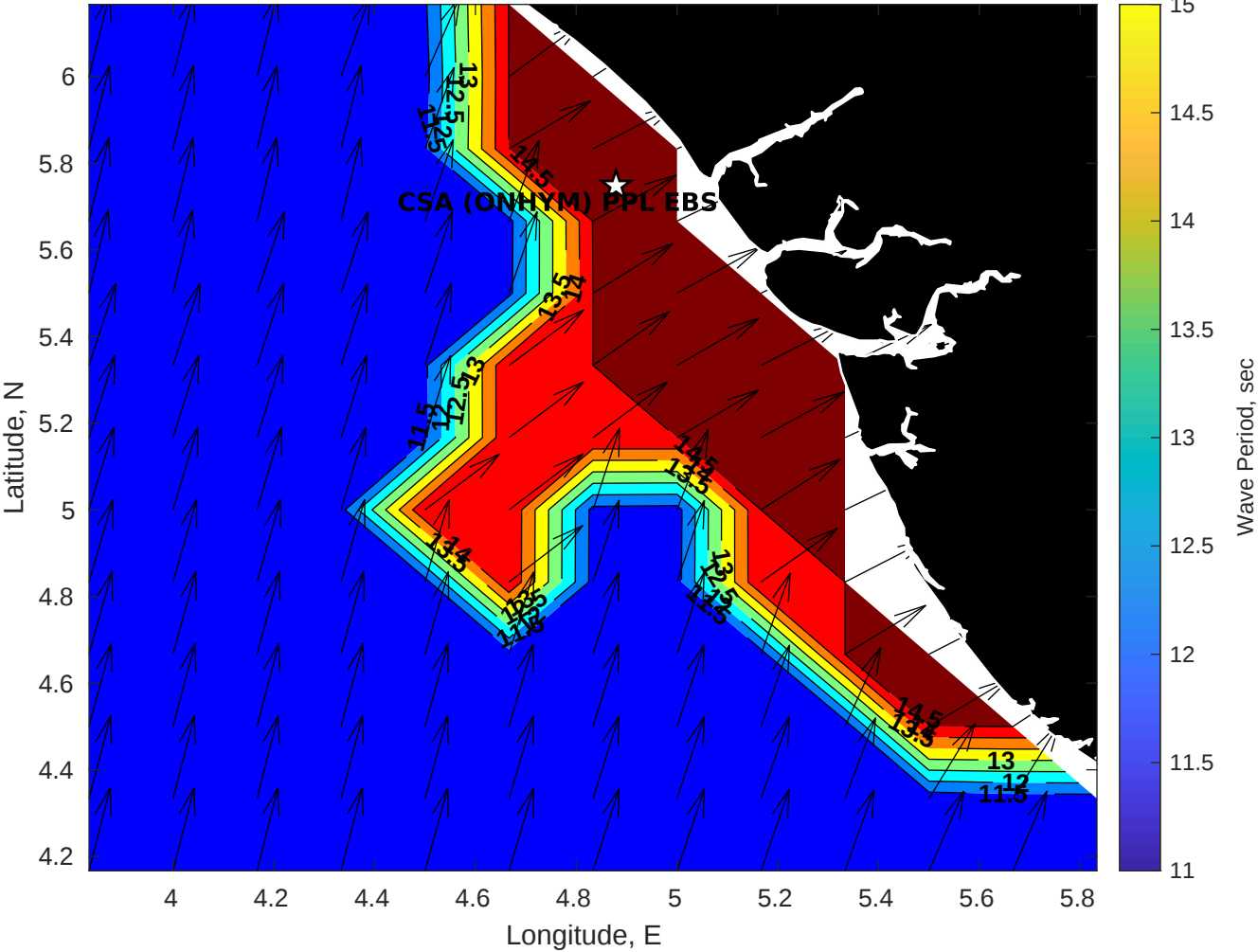
GFS Wave Period (sec) for CSA (ONHYM) PPL EBS - Nigeria at 18-Dec-2025 09:00:00
