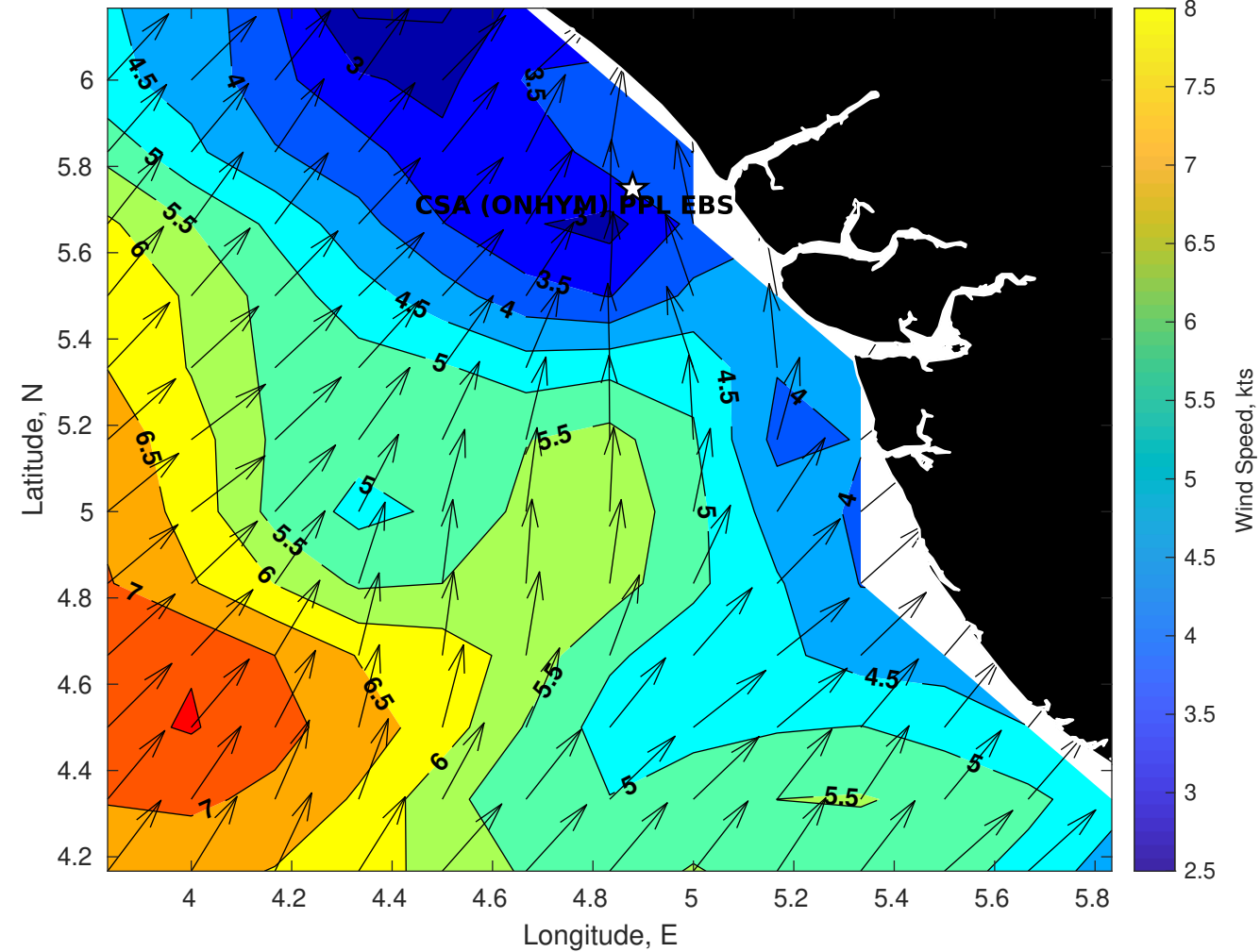
GFS Winds (kts) for CSA (ONHYM) PPL EBS - Nigeria at 18-Dec-2025 09:00:00
