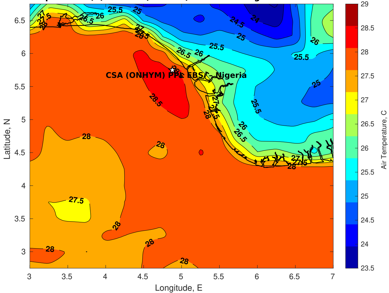
Air Temperature (C) for CSA (ONHYM) PPL EBS - Nigeria at 18-Dec-2025
