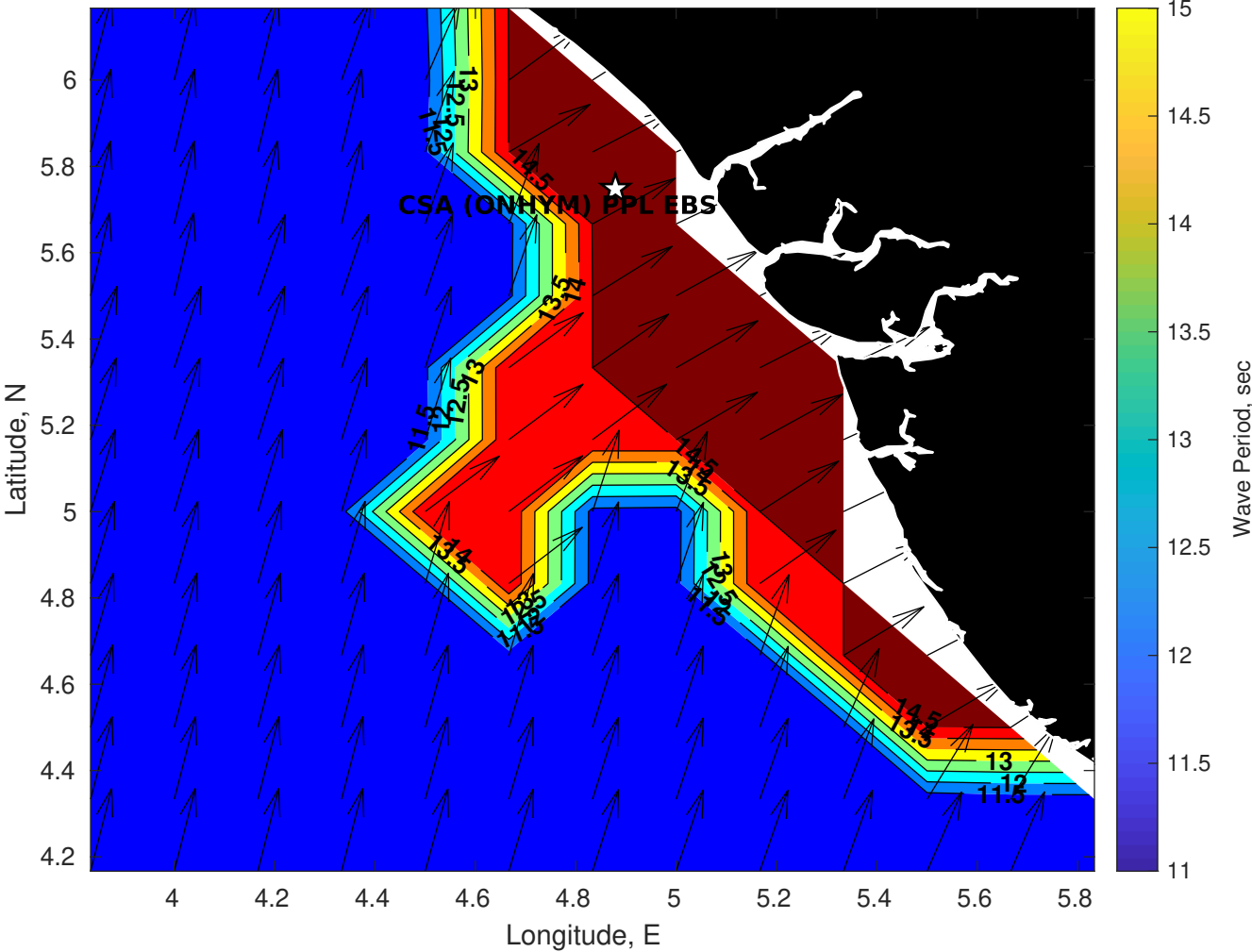
GFS Wave Period (sec) for CSA (ONHYM) PPL EBS - Nigeria at 18-Dec-2025 09:00:00
