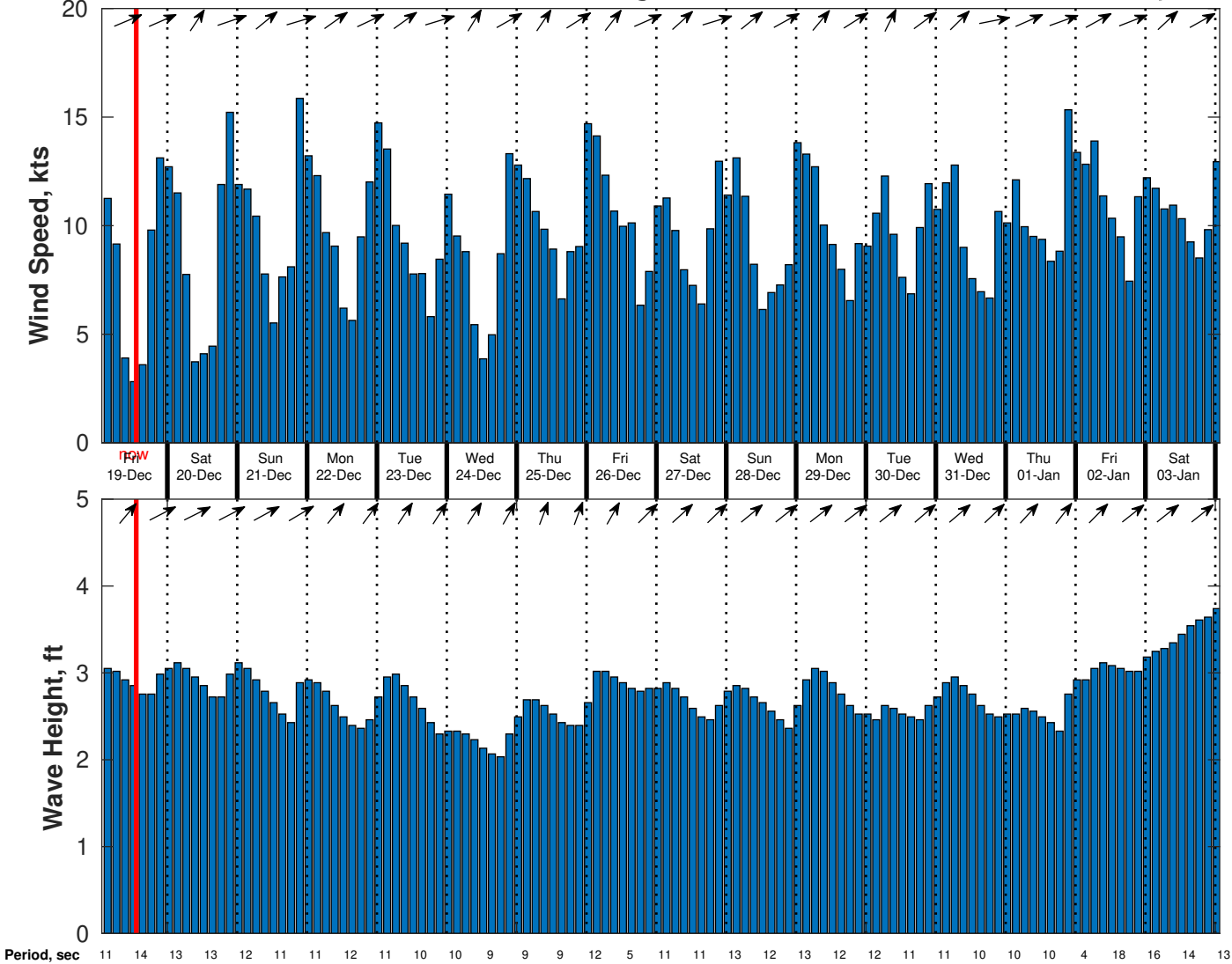
Wind & Wave Forecast for CSA (ONHYM) PPL EBS - Nigeria from 18-Dec-2025 02:00:00 to 03-Jan-2026 02:00:00
