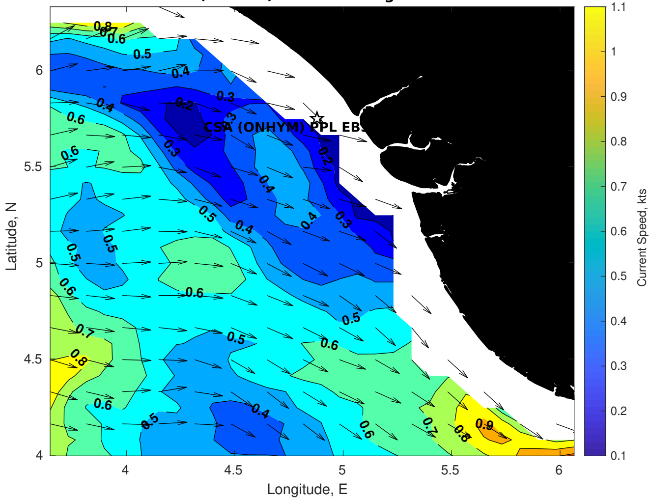
Surface Currents for CSA (ONHYM) PPL EBS - Nigeria at 17-Dec-2025 00:00:00
