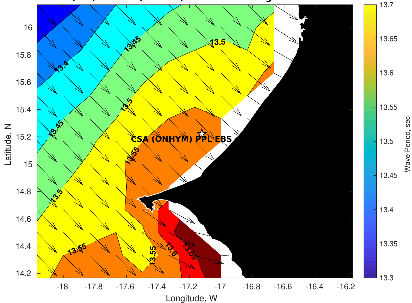
GFS Wave Period (sec) for CSA (ONHYM) PPL EBS - Senegal at 18-Dec-2025 09:00:00
