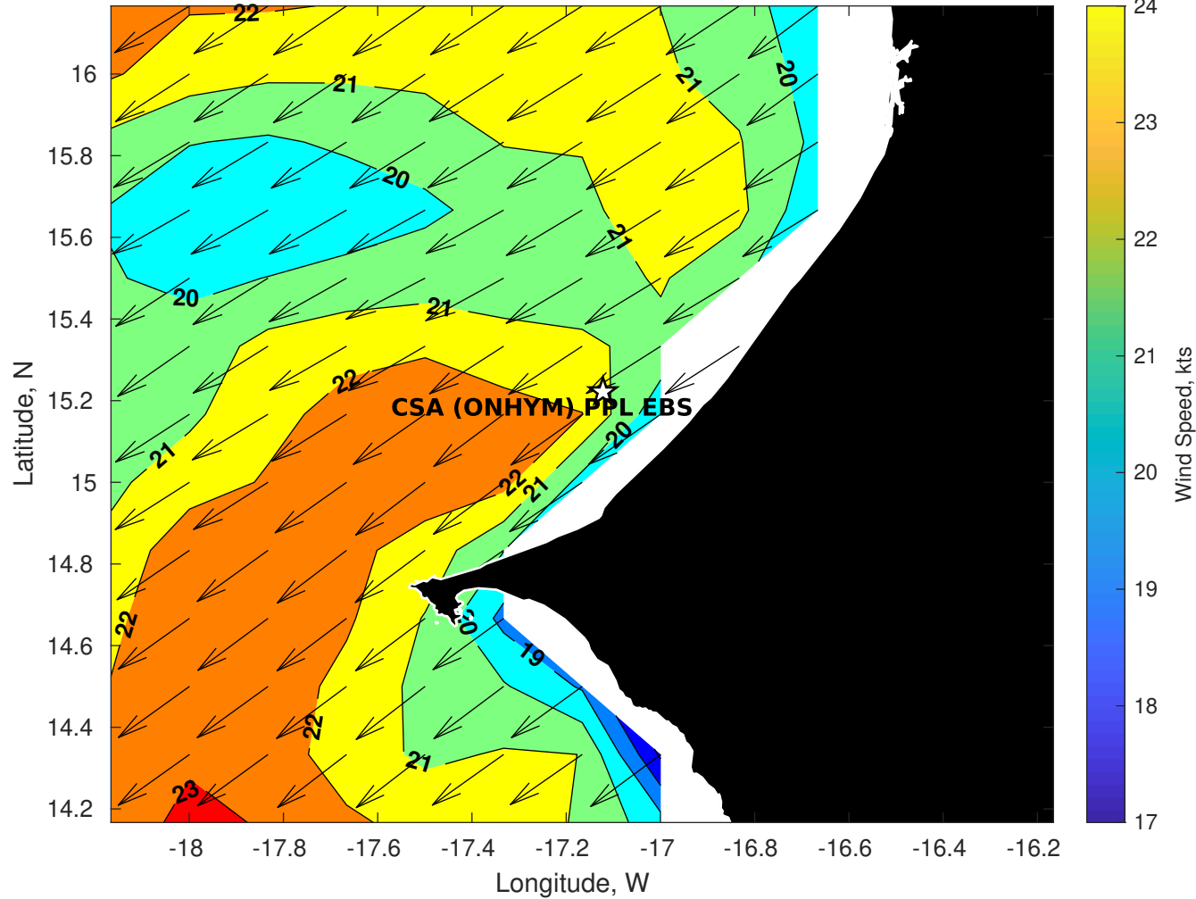
GFS Winds (kts) for CSA (ONHYM) PPL EBS - Senegal at 18-Dec-2025 09:00:00
