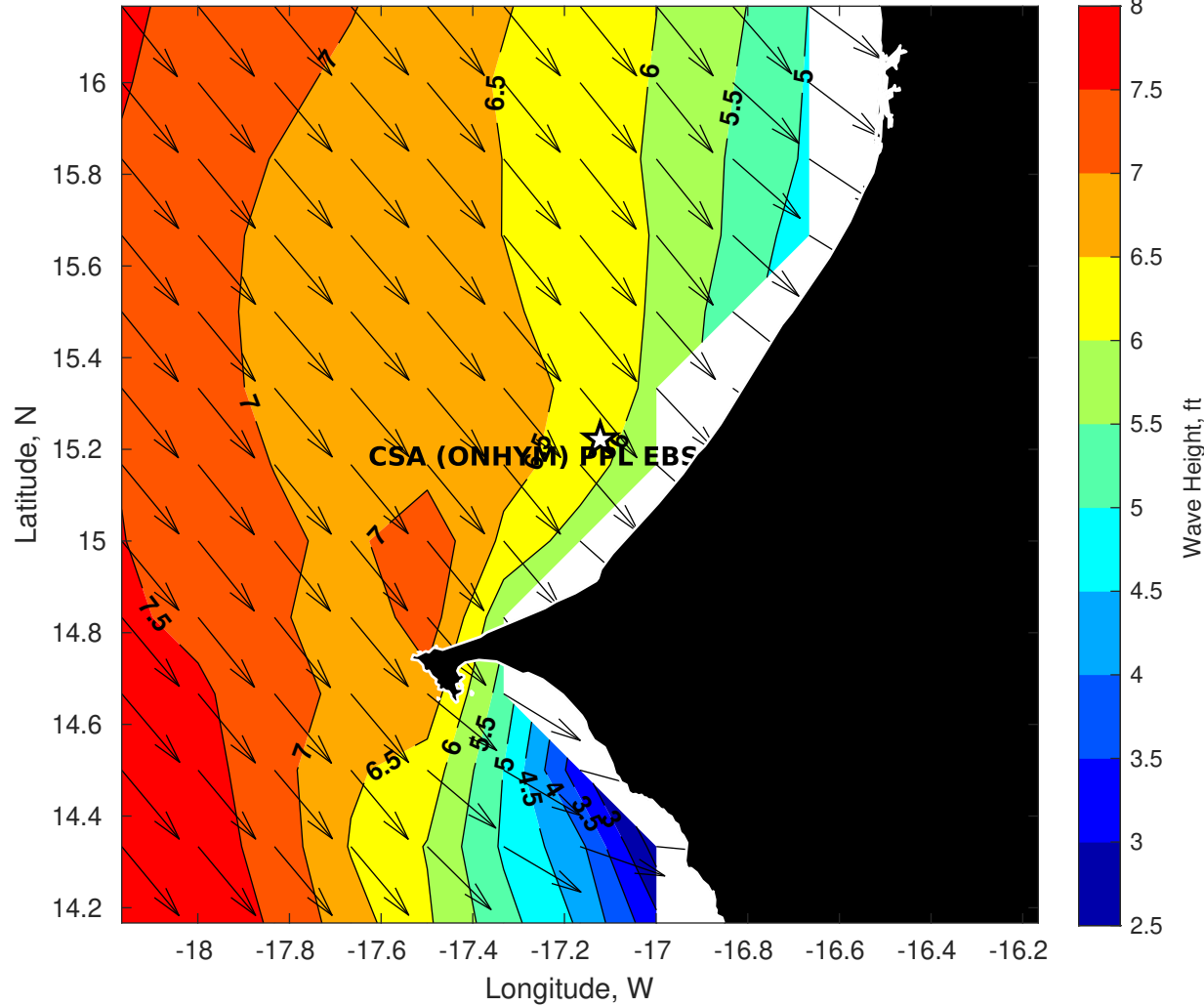
GFS Wave Height (ft) for CSA (ONHYM) PPL EBS - Senegal at 18-Dec-2025 09:00:00
