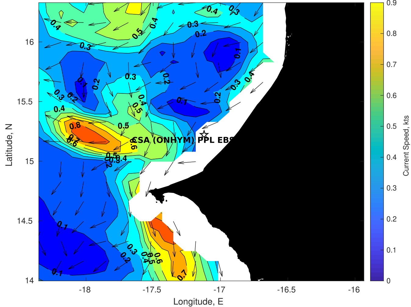
Surface Currents for CSA (ONHYM) PPL EBS - Senegal at 17-Dec-2025 00:00:00
