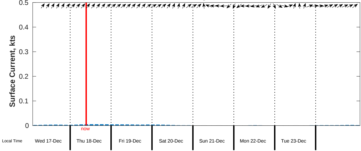
Surface Current Forecast for CSA (ONHYM) PPL EBS - Senegal from 17-Dec-2025 00:00:00 to 25-Dec-2025 00:00:00
