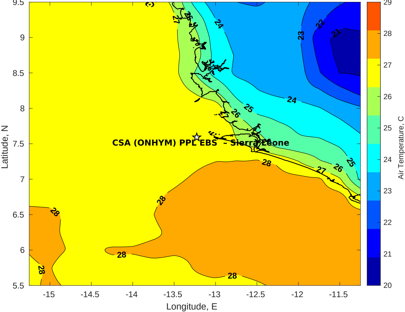
Air Temperature (C) for CSA (ONHYM) PPL EBS - Sierra Leone at 18-Dec-2025
