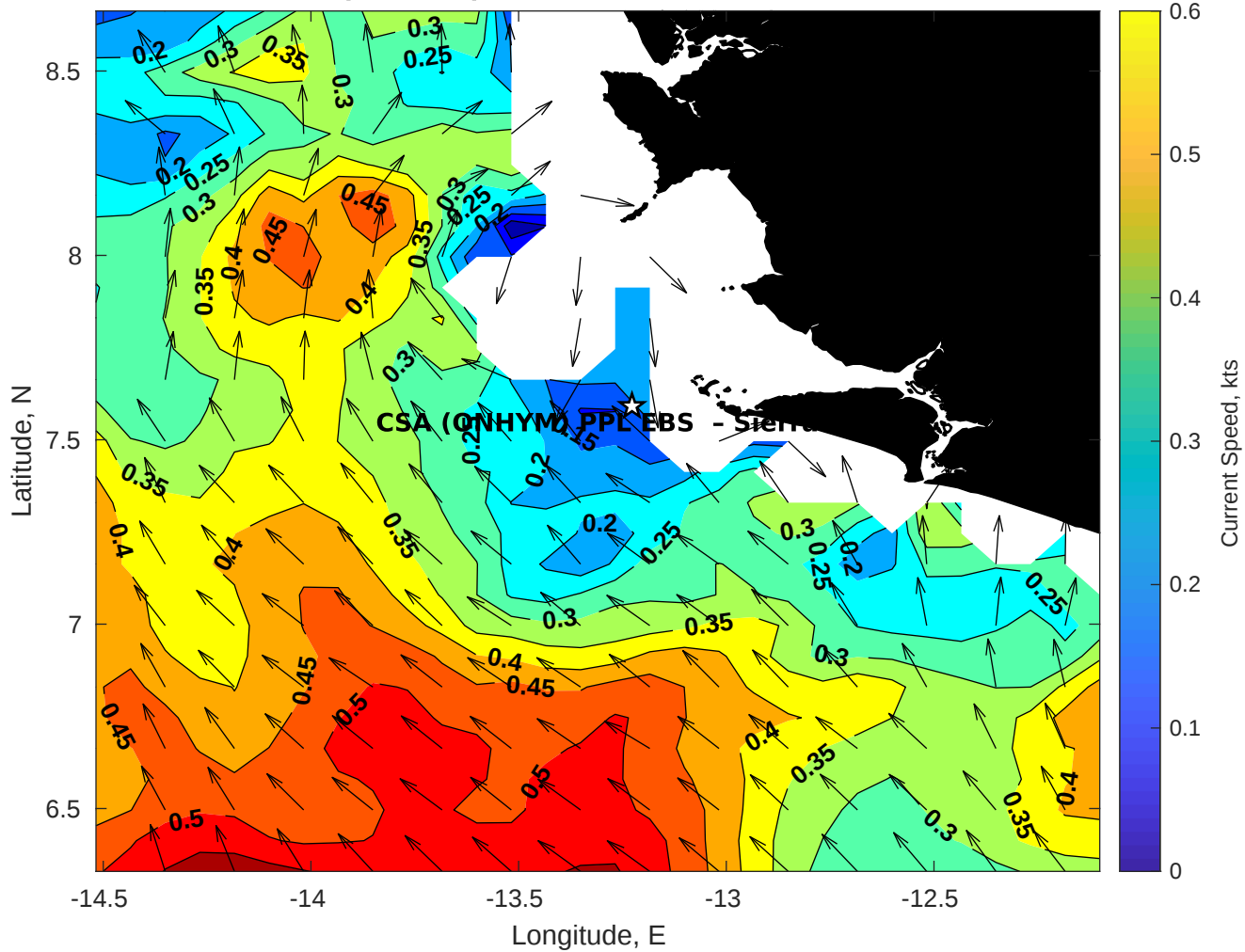
Surface Currents for CSA (ONHYM) PPL EBS - Sierra Leone at 17-Dec-2025 00:00:00
