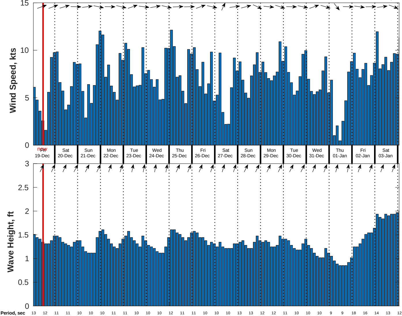
Wind & Wave Forecast for CSA (ONHYM) PPL EBS - Sierra Leone from 18-Dec-2025 01:00:00 to 03-Jan-2026 01:00:00
