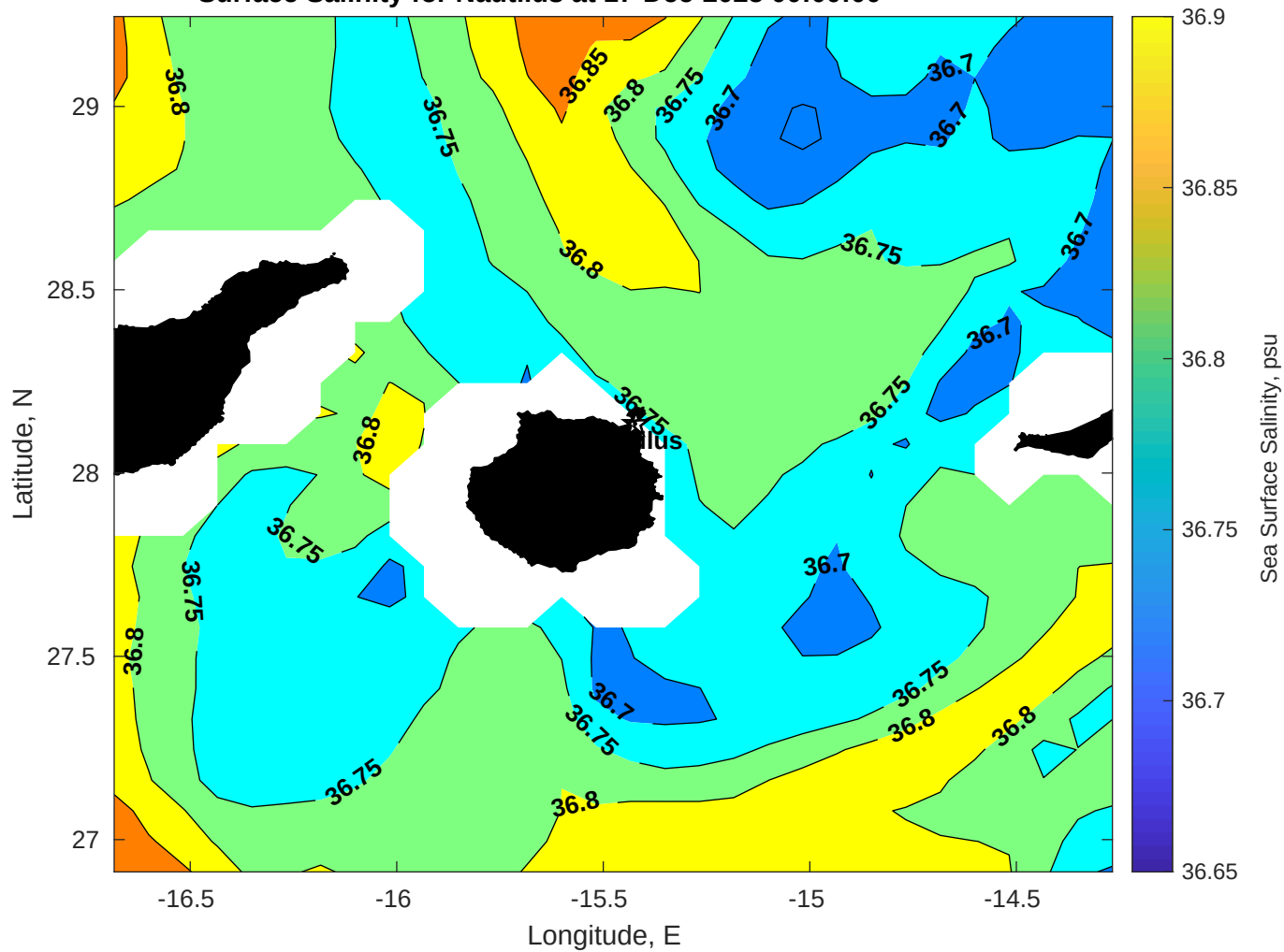
Surface Salinity for Nautilus at 17-Dec-2025 00:00:00
