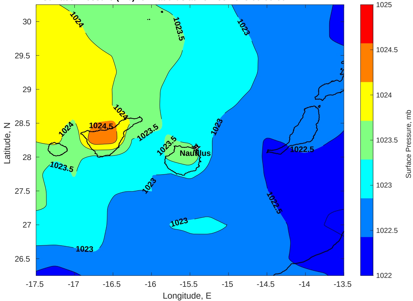
Surface Pressure (mb) for Nautilus at 19-Dec-2025 00:00:00
