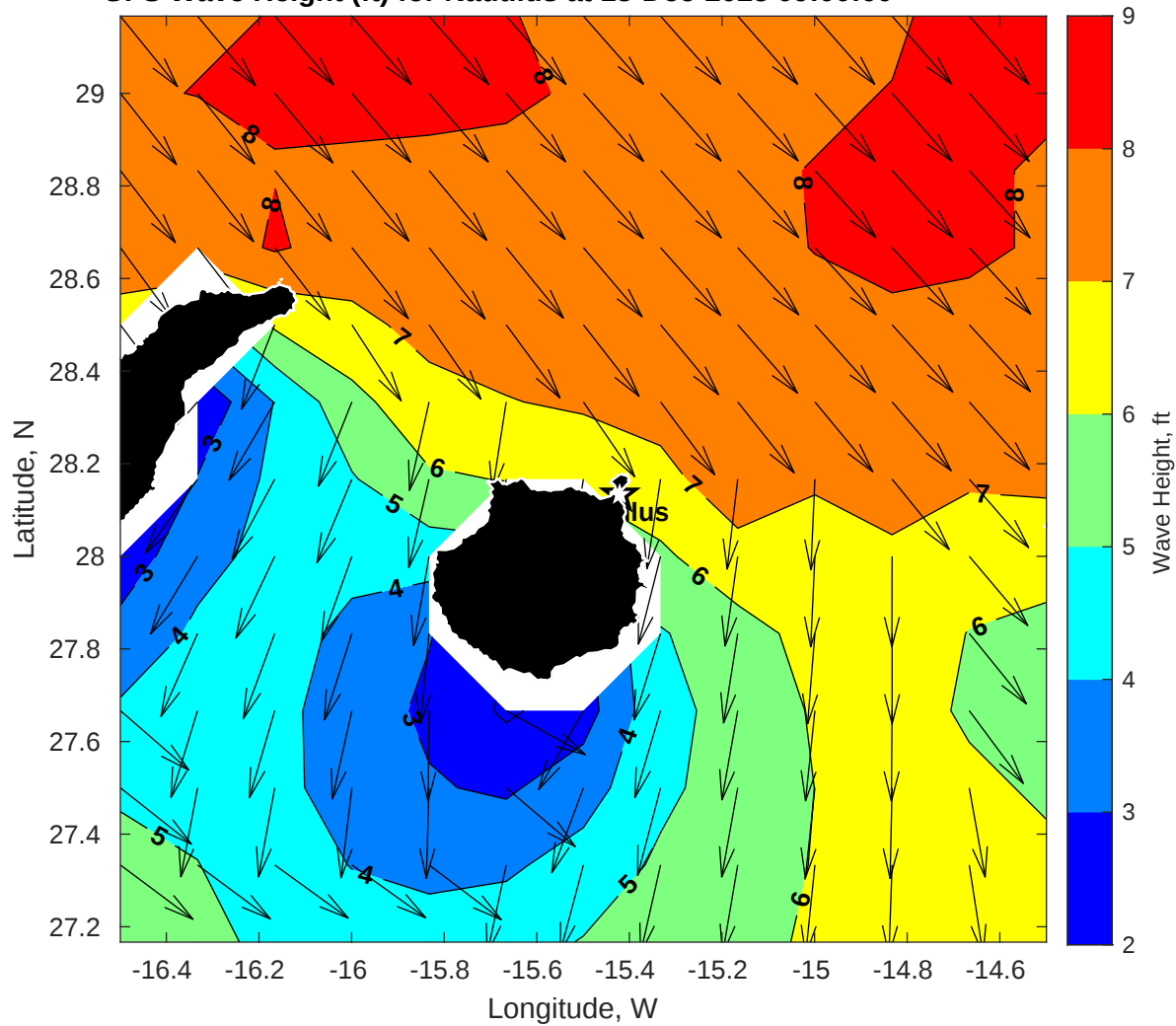
GFS Wave Height (ft) for Nautilus at 18-Dec-2025 09:00:00
