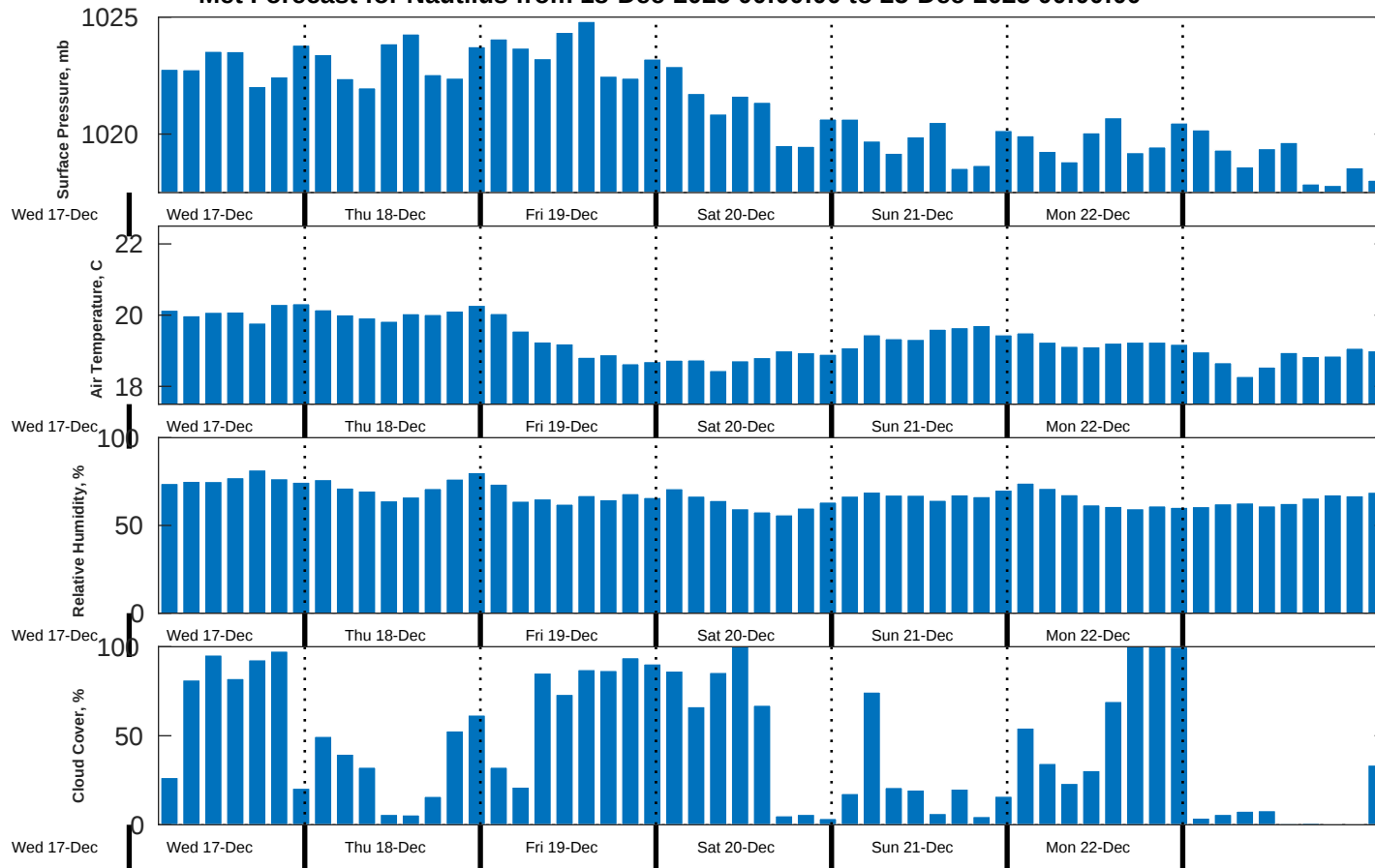
Met Forecast for Nautilus from 18-Dec-2025 00:00:00 to 25-Dec-2025 00:00:00
