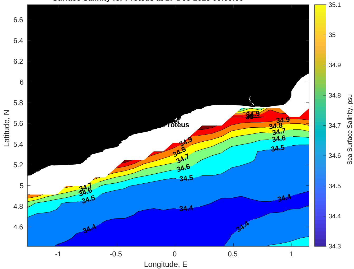
Surface Salinity for Proteus at 17-Dec-2025 00:00:00
