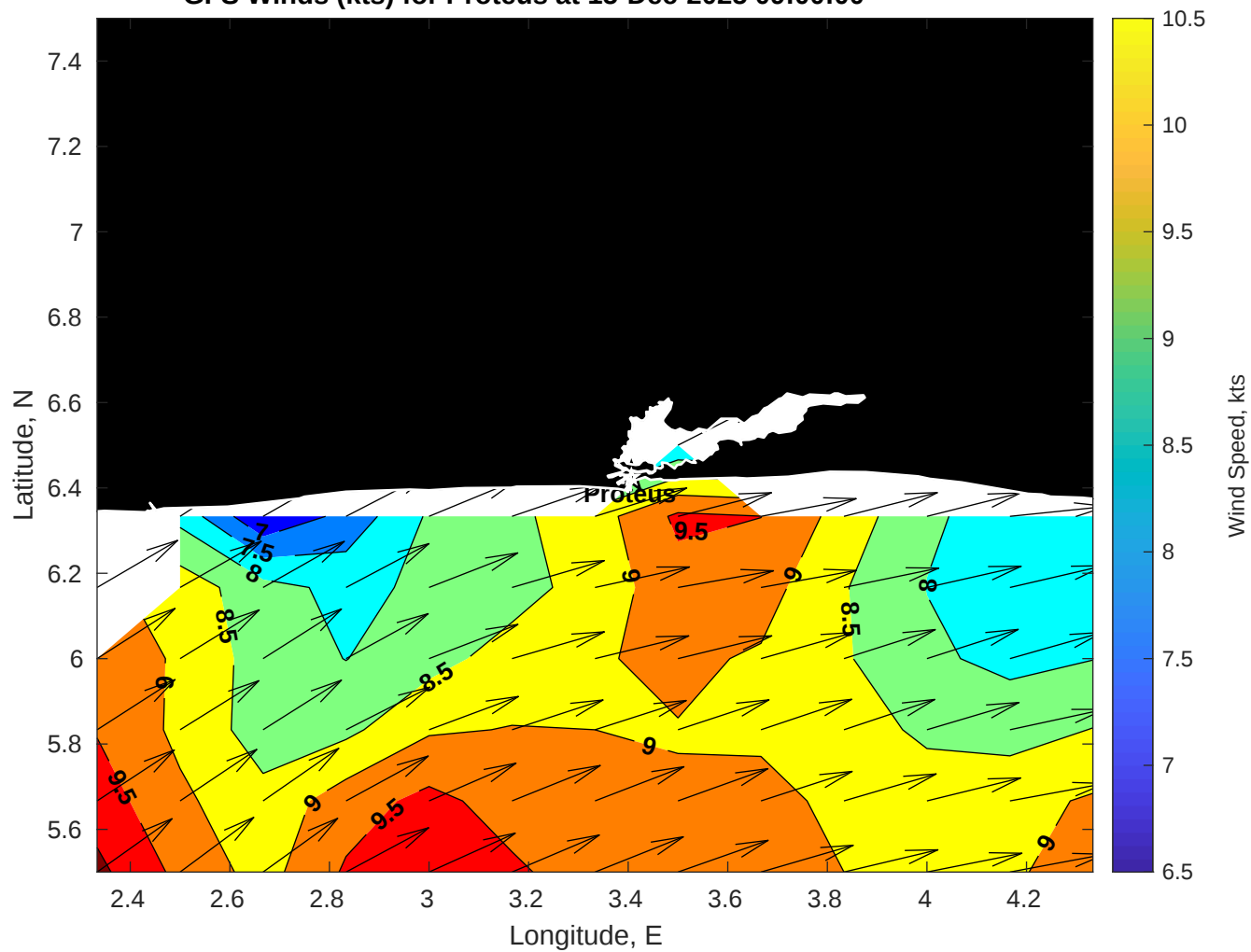
GFS Winds (kts) for Proteus at 15-Dec-2025 09:00:00
