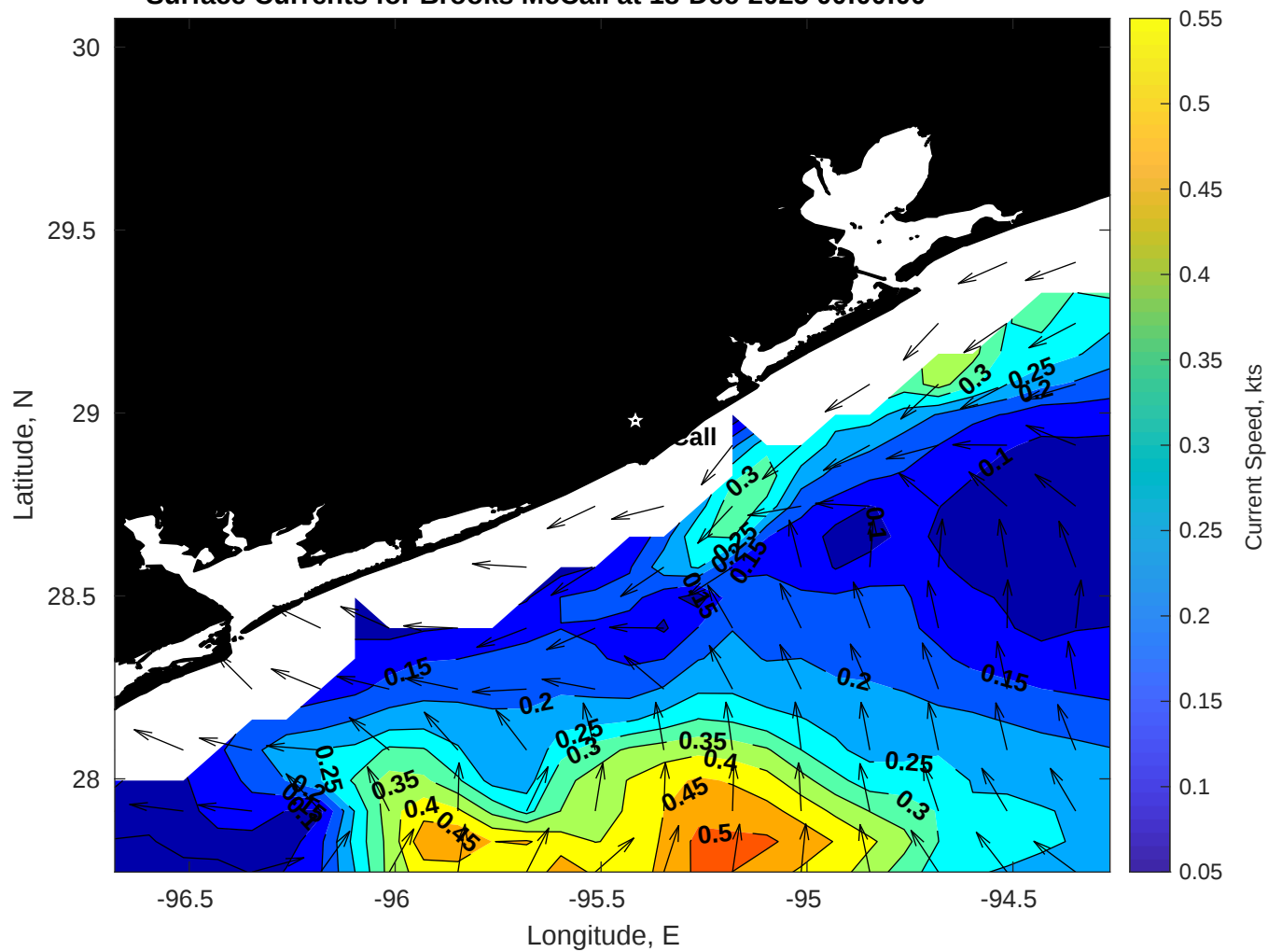
Surface Currents for Brooks McCall at 18-Dec-2025 00:00:00
