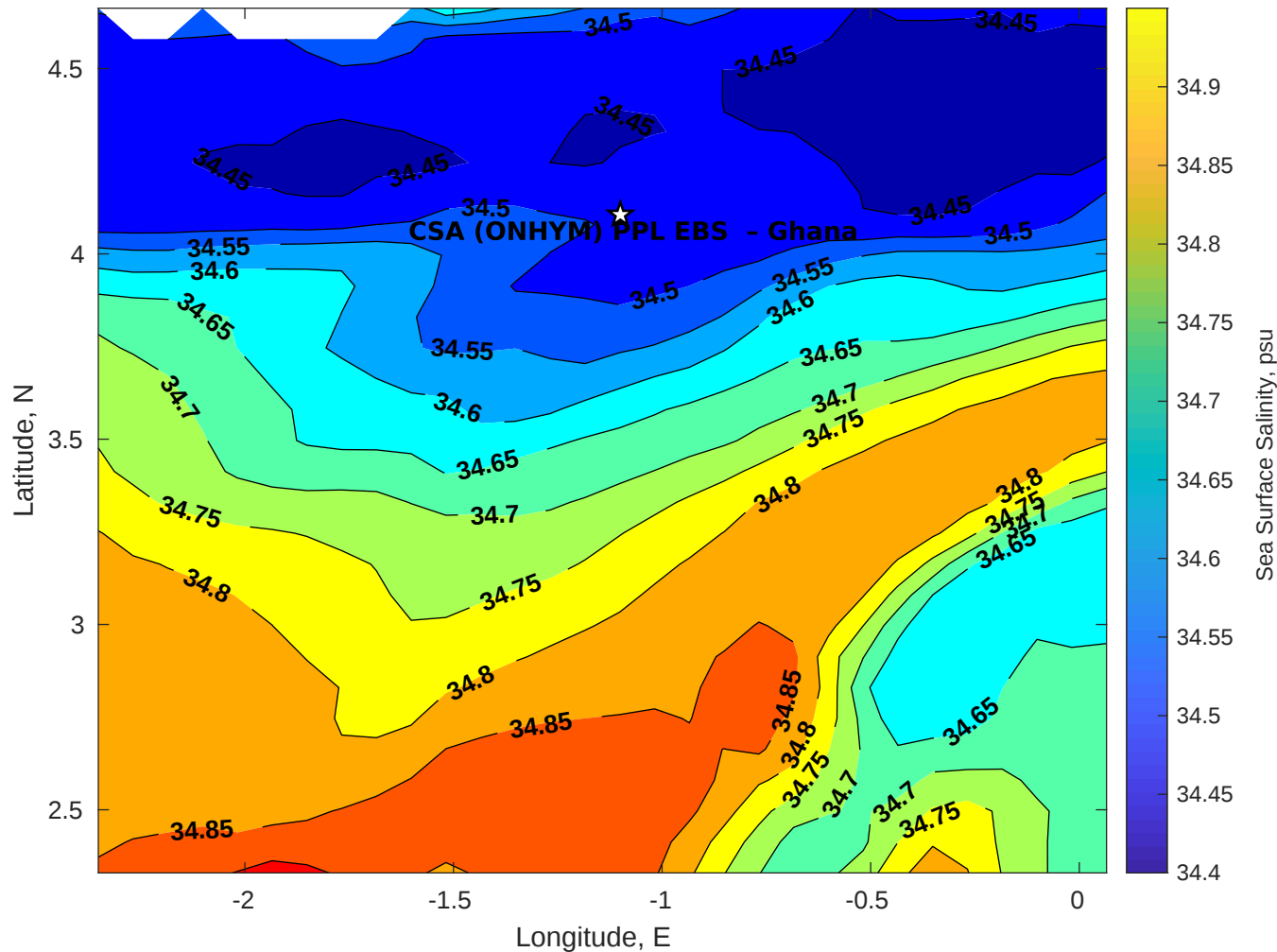
Surface Salinity for CSA (ONHYM) PPL EBS - Ghana at 18-Dec-2025 00:00:00
