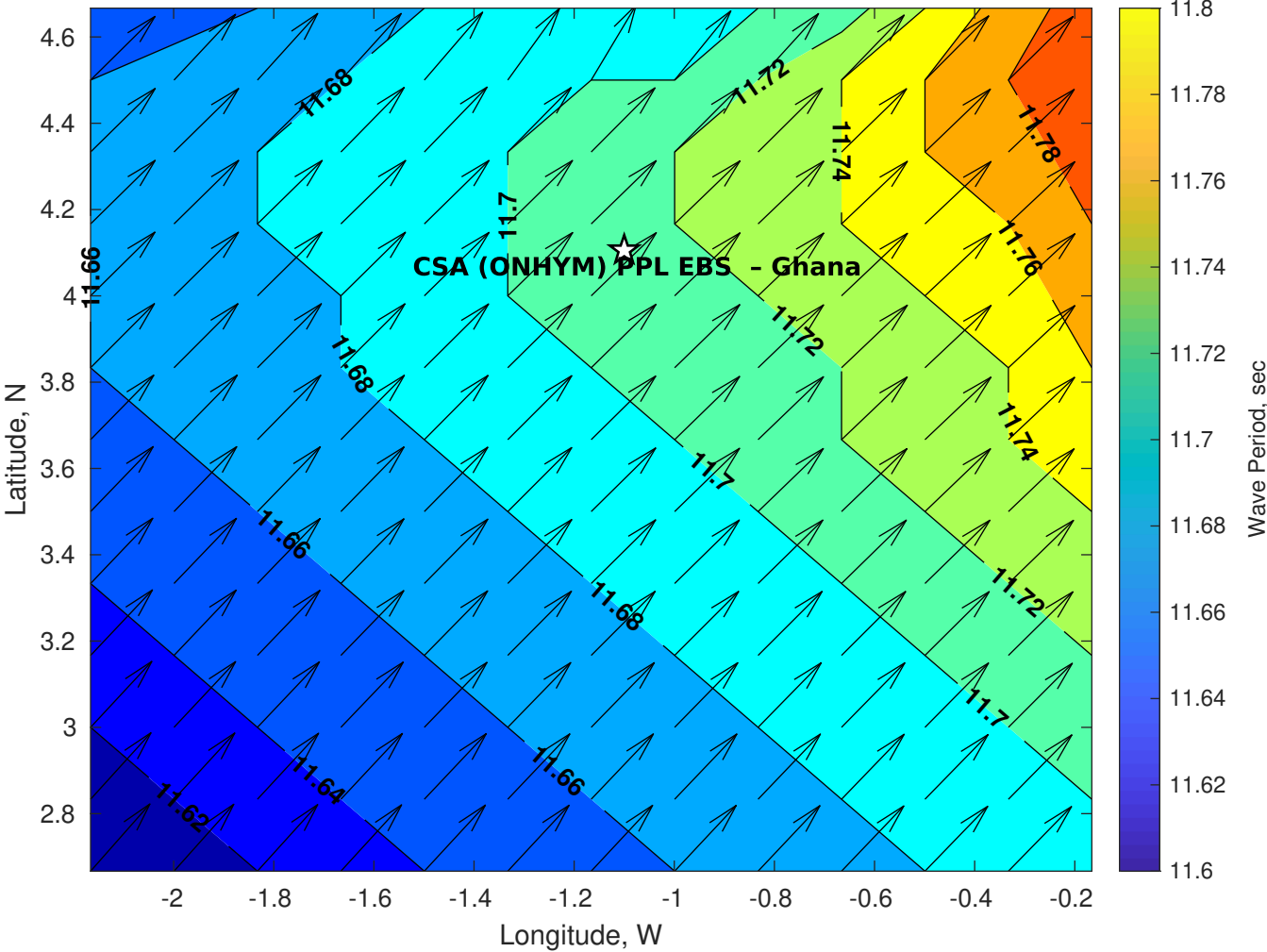
GFS Wave Period (sec) for CSA (ONHYM) PPL EBS - Ghana at 19-Dec-2025 09:00:00
