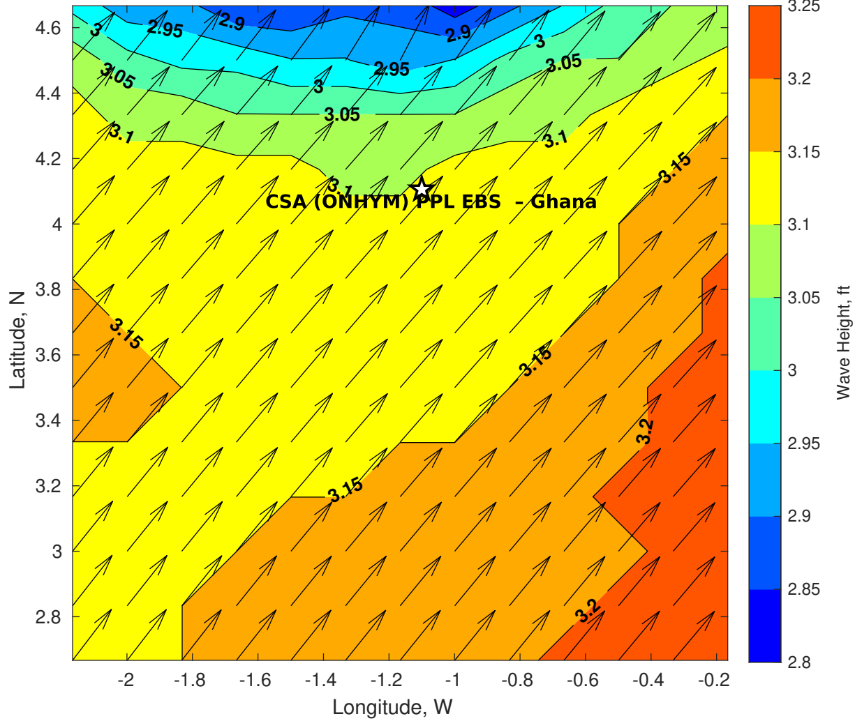
GFS Wave Height (ft) for CSA (ONHYM) PPL EBS - Ghana at 19-Dec-2025 09:00:00
