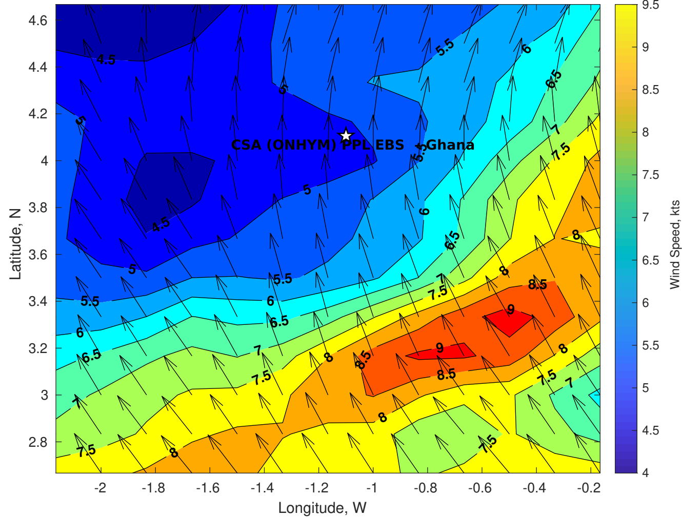
GFS Winds (kts) for CSA (ONHYM) PPL EBS - Ghana at 19-Dec-2025 09:00:00
