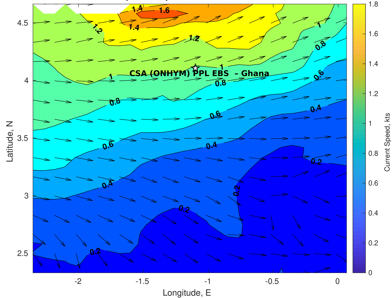
Surface Currents for CSA (ONHYM) PPL EBS - Ghana at 18-Dec-2025 00:00:00
