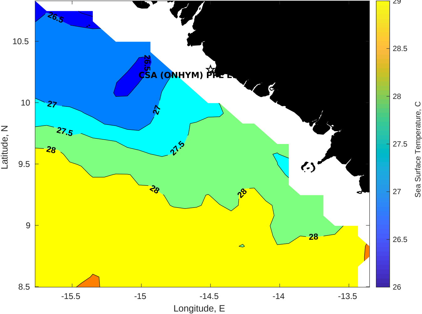
SST for CSA (ONHYM) PPL EBS - Guinea at 18-Dec-2025 00:00:00
